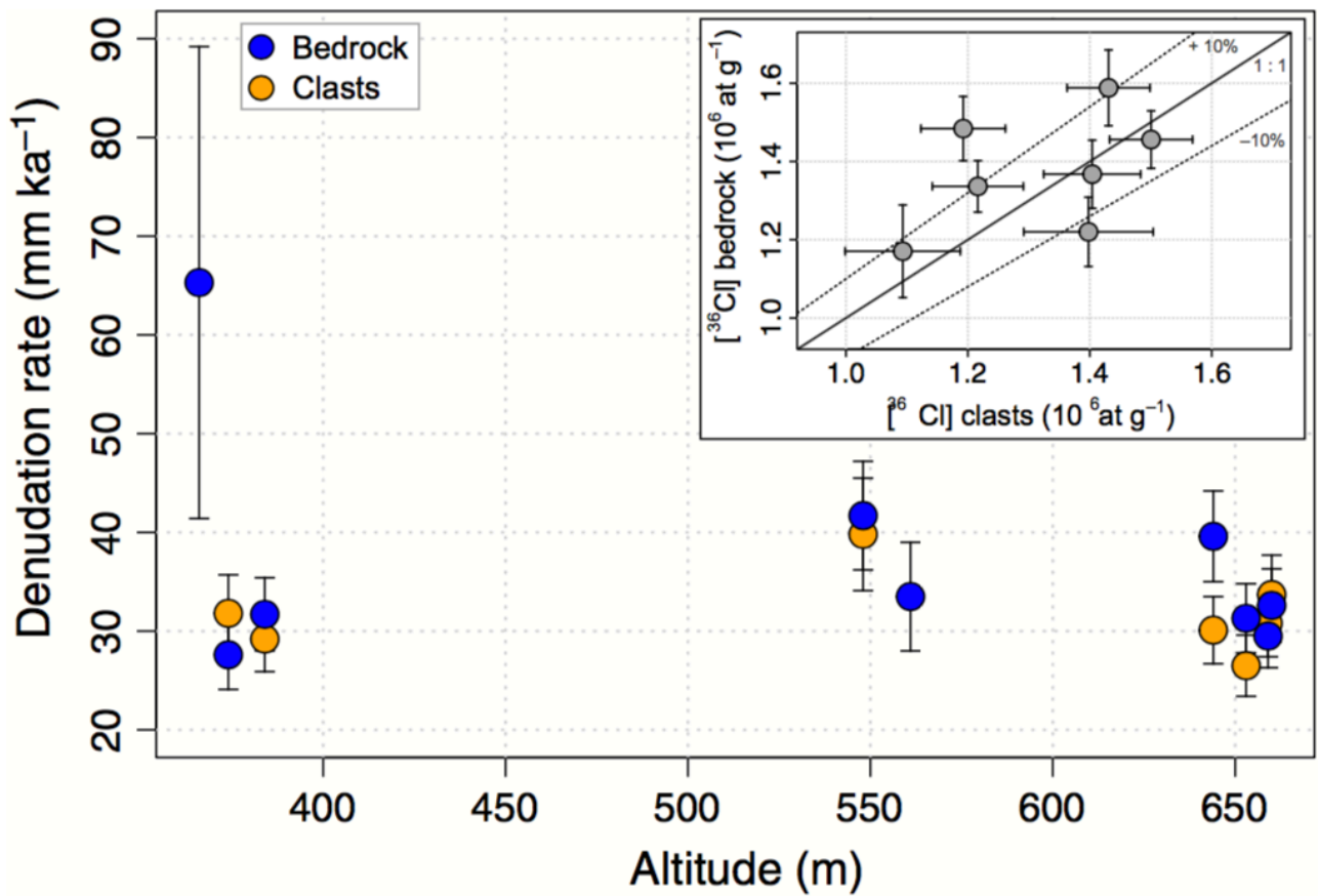
Figure 4 - Denudation rates for surface samples (bedrock or clasts) in the Petit Luberon as a function of the elevation of the sampling site. The inset shows the 36 Cl concentrations in clasts and bedrock samples.
