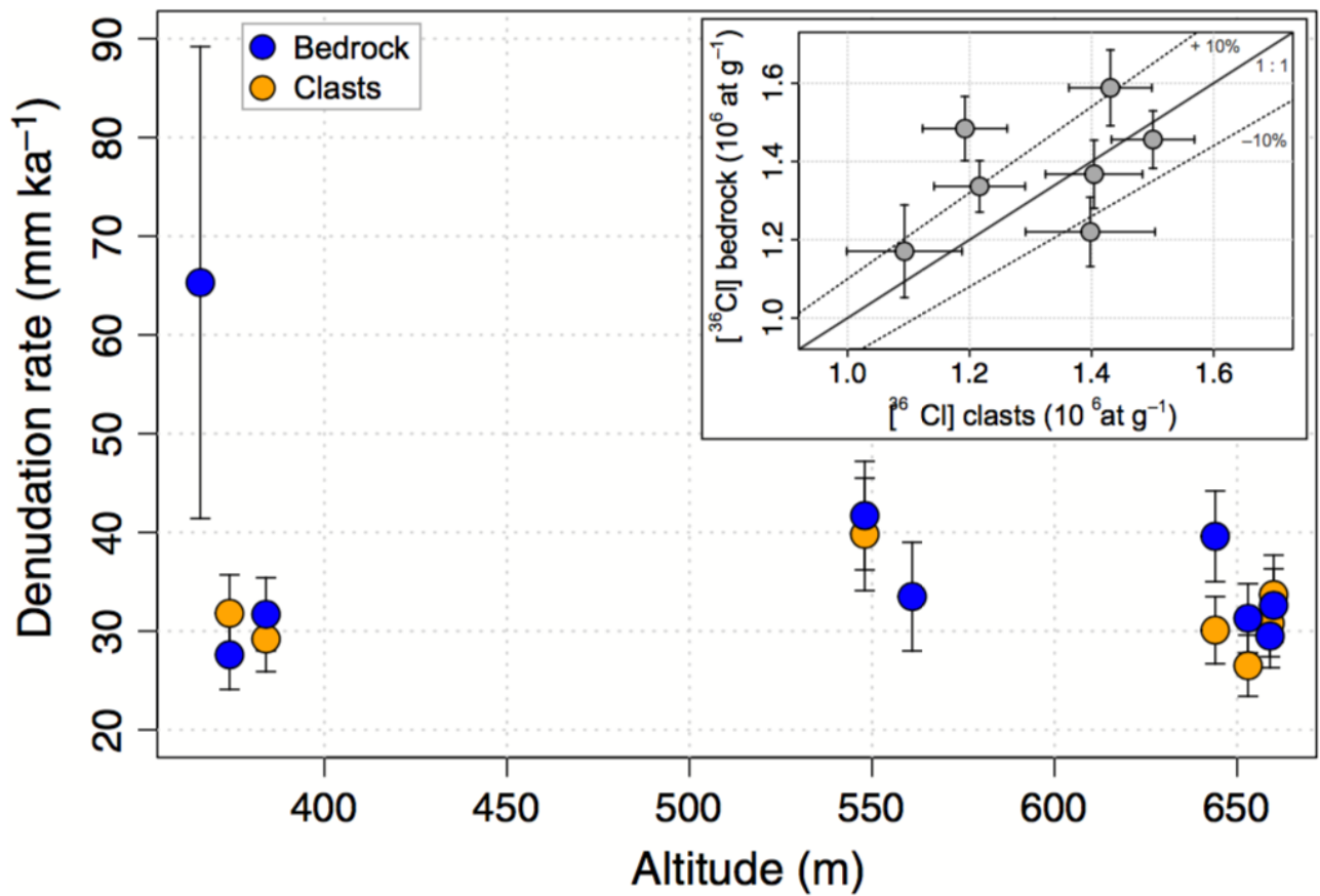
Figure 4 - Denudation rates for surface samples (bedrock or clasts) in the Petit Luberon as a function of the elevation of the sampling site. The inset shows the ^{36}\text{Cl} concentrations in clasts and bedrock samples.
