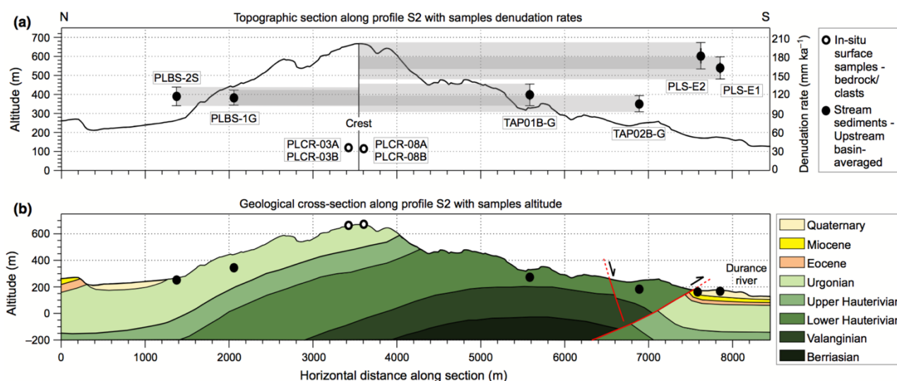
Figure 6 – A: North South topographic profile (see figure 2 for location) through the central part of the Petit Luberon with measured denudation rates. B: Geological cross section across the Petit Luberon anticline. The northern flank is characterized by homogeneously northward dipping strata and a single lithology whereas the geological context of the southern flank is more complex.
