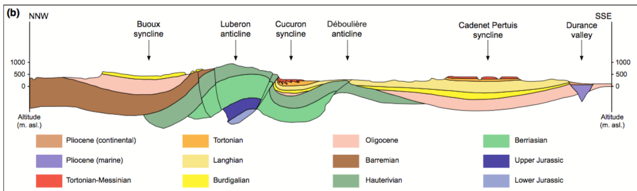
Figure 1 – A: Geological map of South-Eastern France (modified from Molliex et al. , 2011) showing the principal faults and ranges in Provence. The square indicates the location of the Petit Luberon. B: Geological section S through the Grand Luberon mountain (modified from Clauzon et al. , 2011).
