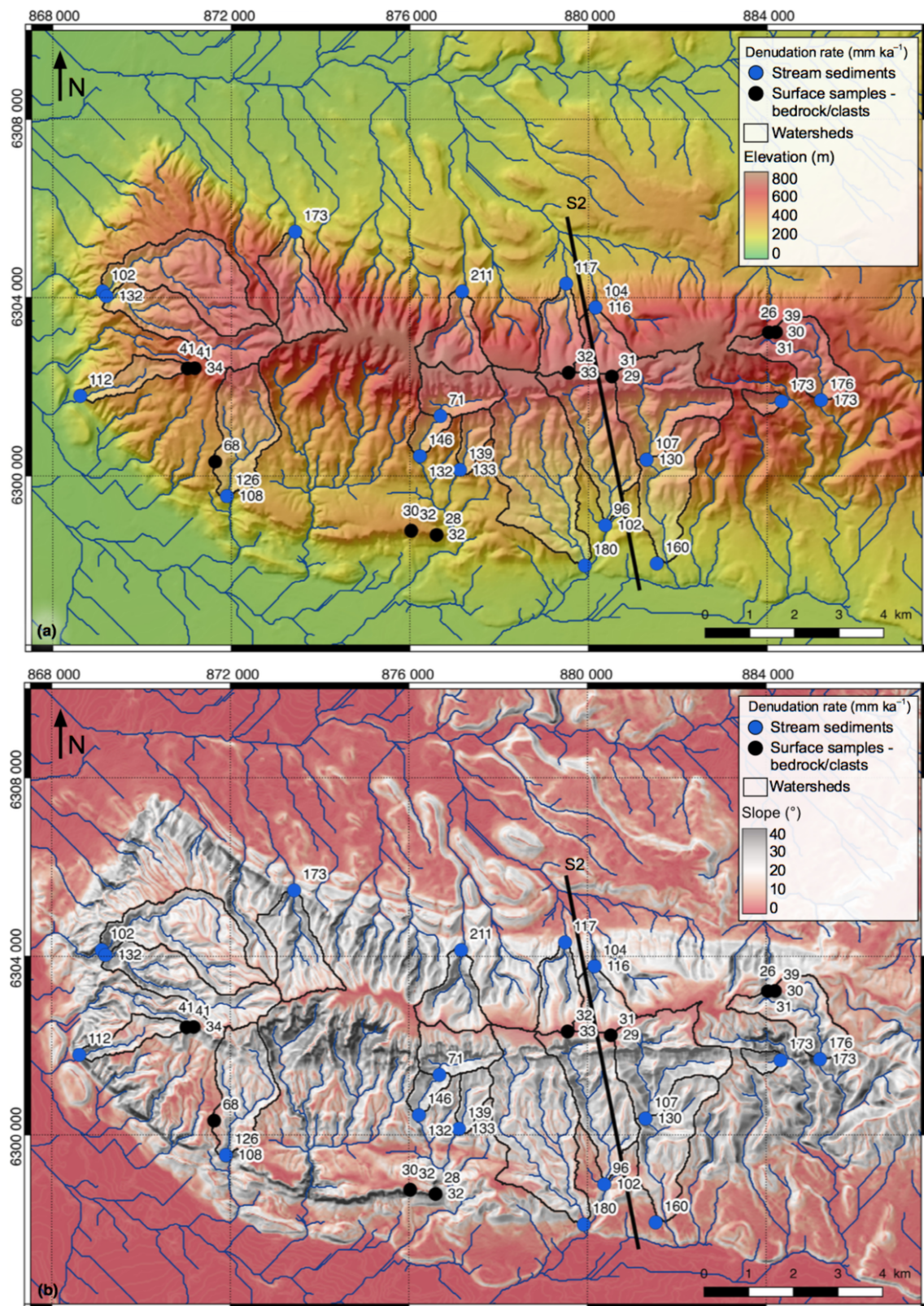
Figure 2 – A: Topographic map of the Petit Luberon with sampling locations and denudation rates (in \text{mm/ka} ). See figure 1 for location. Light blue shading indicates the watersheds corresponding to stream sediments. Black line indicates the location of the topographic and geologic section from figure 6A. B: Slope map of the Petit Luberon highlighting the flat summit surface of the range.
