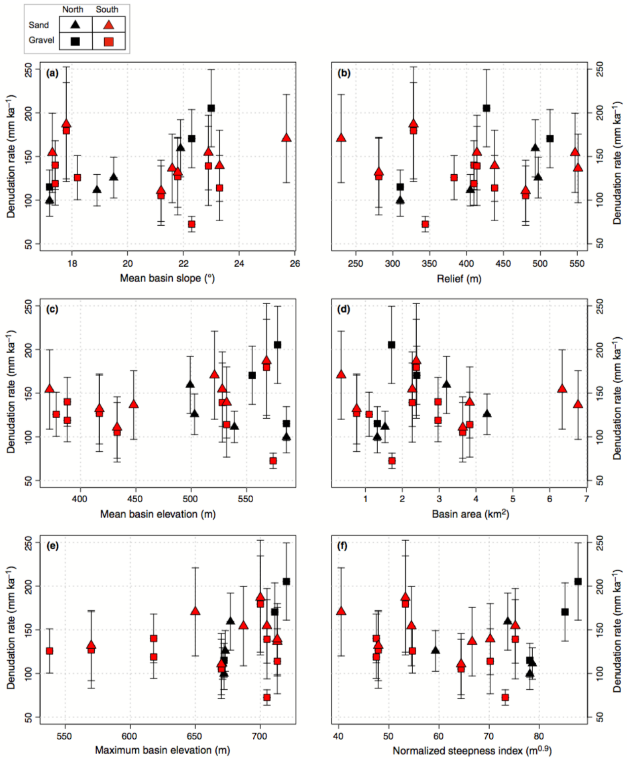
Figure 5 - Catchment-averaged denudation rates in the Petit Luberon flanks as a function of various morphological parameters. Symbol color indicates the location of the catchment (southern or northern flank) and symbol shape indicates the grain size of the sample (sand or gravel).
