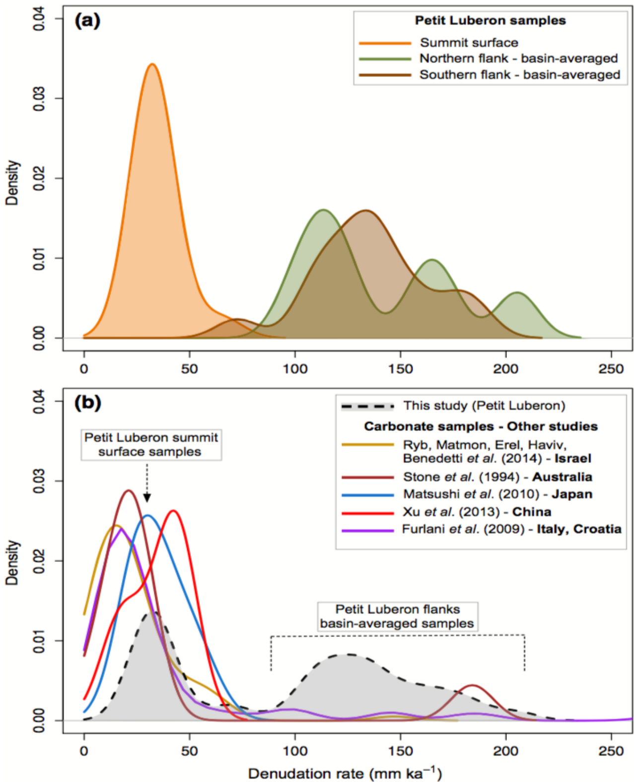
Figure 3 – A: Distribution of denudation rates on the Petit Luberon and in other carbonate landscapes (kernel density function). A: Distribution of denudation rates on the Petit Luberon depending on the sampling location (crest, northern flank and southern flank). B: Comparison of denudation rates in the Petit Luberon with results from previous similar studies in carbonate landscapes.
