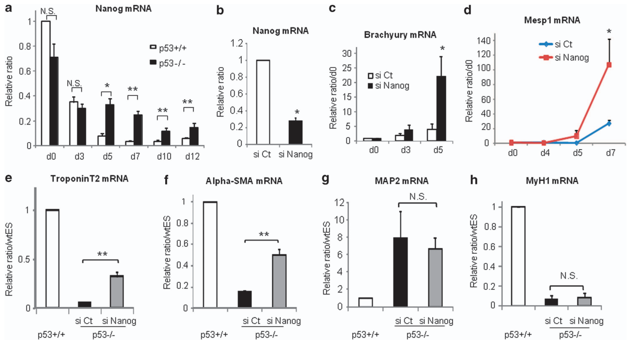
Figure 8 Role of p53-dependent Nanog repression on ESC differentiation. (a) p53^{-/-} ESCs ( p53^{-/-} ) and their wild-type counterparts ( p53^{+/+} ) were induced to differentiate until day 12 and analyzed for endogenous Nanog expression at various time from day 0 to 12, as indicated. mRNAs were extracted and analyzed by real-time RT-PCR. Results are expressed in arbitrary units, with the values of wild-type control ESCs at day 0 taken as 1, and are the means \pm S.E.M. of at least three independent experiments. (b–h) Undifferentiated p53^{-/-} ESCs were transfected overnight with control siRNAs (si Ct) or anti-Nanog siRNAs (si Nanog) and were kept in undifferentiated conditions (b), or induced to differentiate until day 5 (c), day 7 (d), day 12 (e–g) or day 26 (h) and compared with differentiated p53^{+/+} ESC counterparts. mRNAs were extracted 24 h later (b), at days 0, 3, 5 and 7 (c and d), or after differentiation (e–h), and analyzed by real-time RT-PCR for Nanog (b), Brachyury (c), Mesp1 (d), TroponinT2 (e), Alpha-SMA (f), MAP2 (g) and MyH1 (h) gene expression. Results are expressed in arbitrary units, with the values of si Ct control ESCs taken as 1 (b–d), or with the values of wild-type control ESCs taken as 1 (e–h), and are the means \pm S.E.M. of at least three independent experiments. Significance to values obtained with p53^{+/+} cells or siCt conditions is given as: * P < 0.05 and ** P < 0.01
