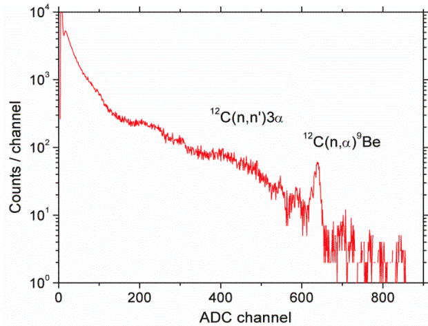
Fig. 4: Typical ISMART SiC diode (here approx. 5 mm × 5 mm) and example of a recorded pulse height spectrum under DT neutron irradiation.
