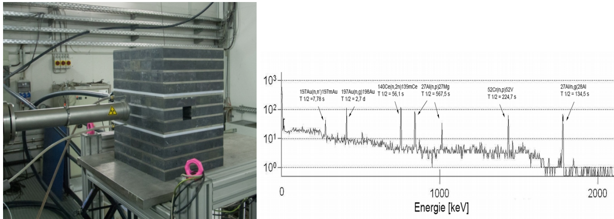
Fig. 2: Experimental setup for testing of activation foils at TUD-NG and example of a recorded gamma ray spectrum with multifoil measurement.
