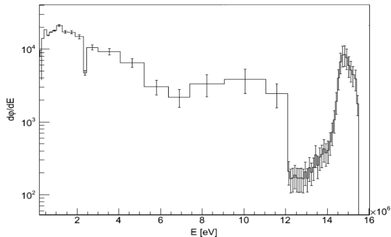
Fig. 3. Unfolded neutron spectrum and uncertainties of the measurement in the HCLL TBM mockup TBM.
