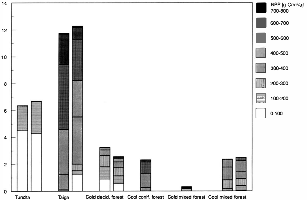
Fig. 1. Comparison of the net primary productivity (npp) areas of northern ecosystem types for the original FBM (right column) and for the coupled model (left column) at current climate, classified into 8 npp classes from 0 to 800 g C m -2 a -1 . Matthews vegetation types are assigned to biome types according to Table 1.
