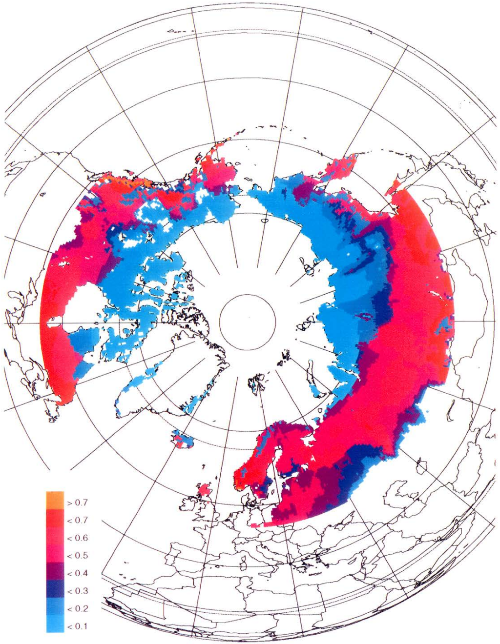
Fig. 2. Geographic pattern of npp in classes from 0 to 0.8 kg C m -2 a -1 of Northern ecosystems (shown only north of 50°N), derived from the coupled model.
