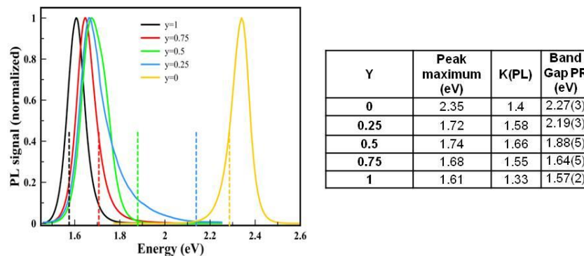
Figure 6. PL peaks for different I/Br ratios in \text{CH}_3\text{NH}_3\text{PbCl}_x(\text{I}_y\text{Br}_{1-y})_{3-x} [14] and PR results [17].
