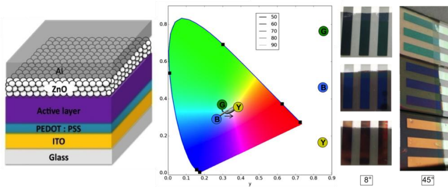
Figure 12. Left : Organic solar cell in a classical architecture. Right : Predicted color as a function of active layer and ZnO thicknesses (An arrow indicates the increase of the active layer thickness) and photograph images of the Green (G), Blue (B) and Yellow (Y) solar cells at 8° and 45° (right) [21].
