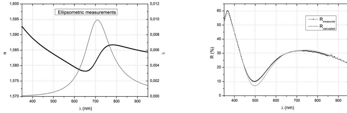
Figure 10. Left : Ellipsometric measurements on heterogeneous layer made of metallic nanoparticles embedded in PVP polymer. Right : Reflection spectrum measured and calculated by TMM thanks to ellipsometric measurements.
