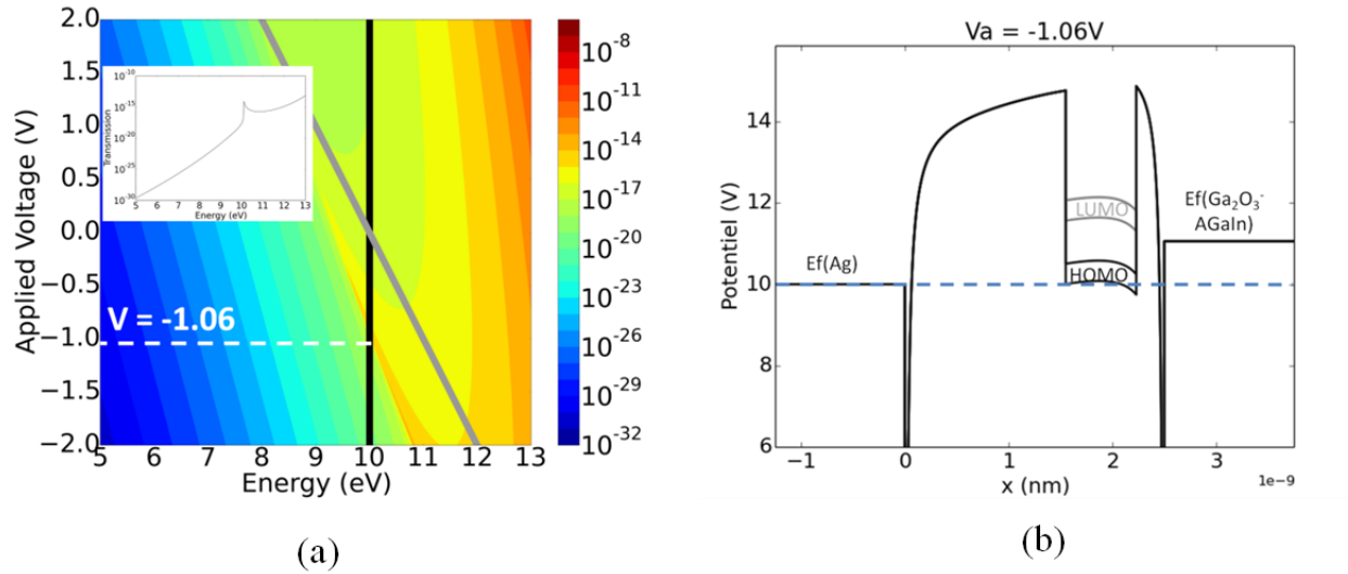
FIG.4. (a) Computed color map of the tunneling probability for the HSC 11 Fc based junction by considering \Gamma_{\text{HOMO}} = \Gamma_{\text{LUMO}} = 0.5 eV. The computations are performed considering only the HOMO of the ferrocene moiety. (b) Potential inside the HSC 11 Fc based molecular diode at V_a = -1.06 V ( \Gamma_{\text{HOMO}} = \Gamma_{\text{LUMO}} = 0.5 eV).
