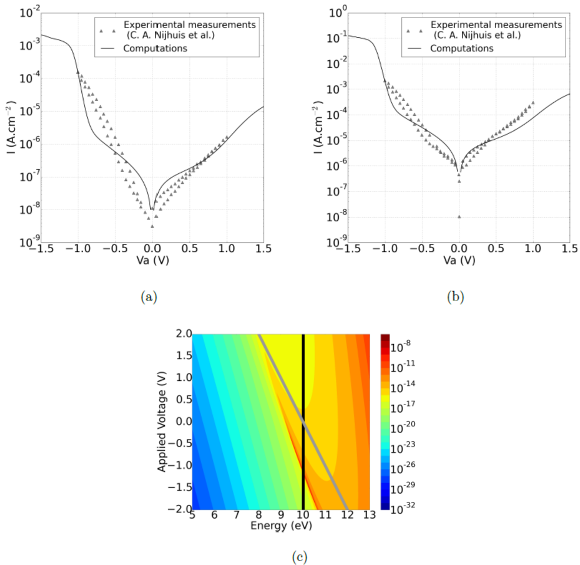
FIG.6. Comparison between computed I(V_a) characteristics and experimental measurement obtained by Nijhuis, Reus and Whitesides 10 for (a) a HSC 11 Fc based molecular junction and (b) a HSC 9 Fc based molecular junction. (c) is a color map of the tunneling probability for the HSC 9 FC based molecular diode ( \Gamma_{\text{HOMO}}=0.57\text{eV} and \Gamma_{\text{LUMO}}=0.6\text{eV} ).
