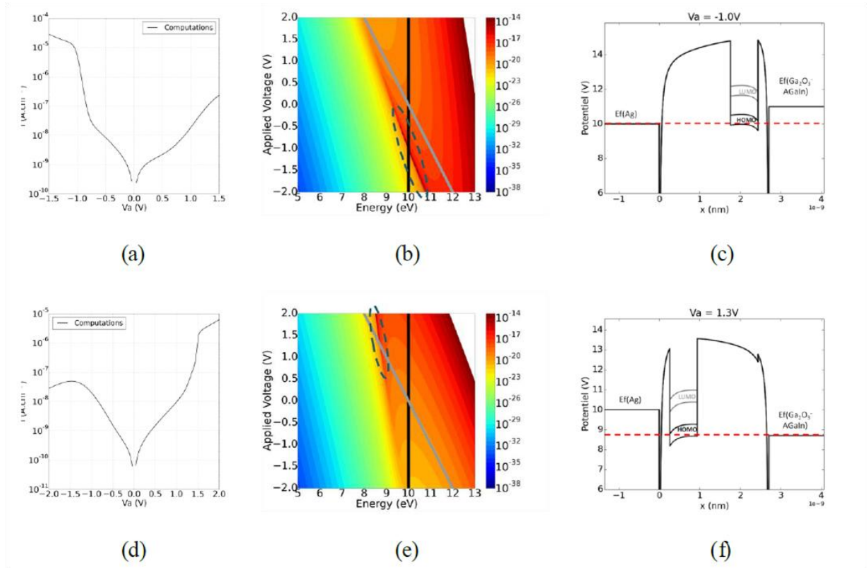
FIG. 7. Computed (a) I(V_a) characteristics, (b) color map of the tunneling probability and (c) potential inside the molecular junction for a HSC 13 Fc based diode. Computed (d) I(V_a) characteristics, (e) color map of the tunneling probability and (f) potential inside the molecular junction for a HSFcC 13 based diode.
