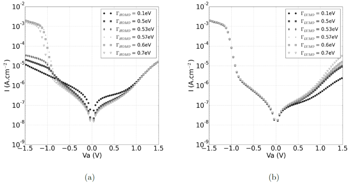
FIG.2. Influence of the the energy level broadening (a) \Gamma_{HOMO} and (b) \Gamma_{LUMO} on the calculated I(V_a) characteristics of a HSC11Fc molecular diode.
