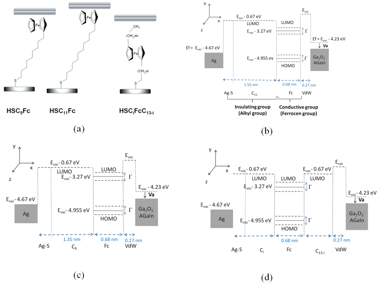
FIG.1. (a) Schematic representation of molecular diodes made of ferrocenyl-containing alkanethiols. It consists in Ag bottom electrodes, SAM of SC 9 Fc, SC 11 Fc or SC i FcC 13-i and Ga 2 O 3 -EGaIn electrodes. Theoretical energy band diagram of molecular diodes made of (b) HSC 11 Fc, (c) HSC 9 FC and (d) HSC i FcC 13-i .
