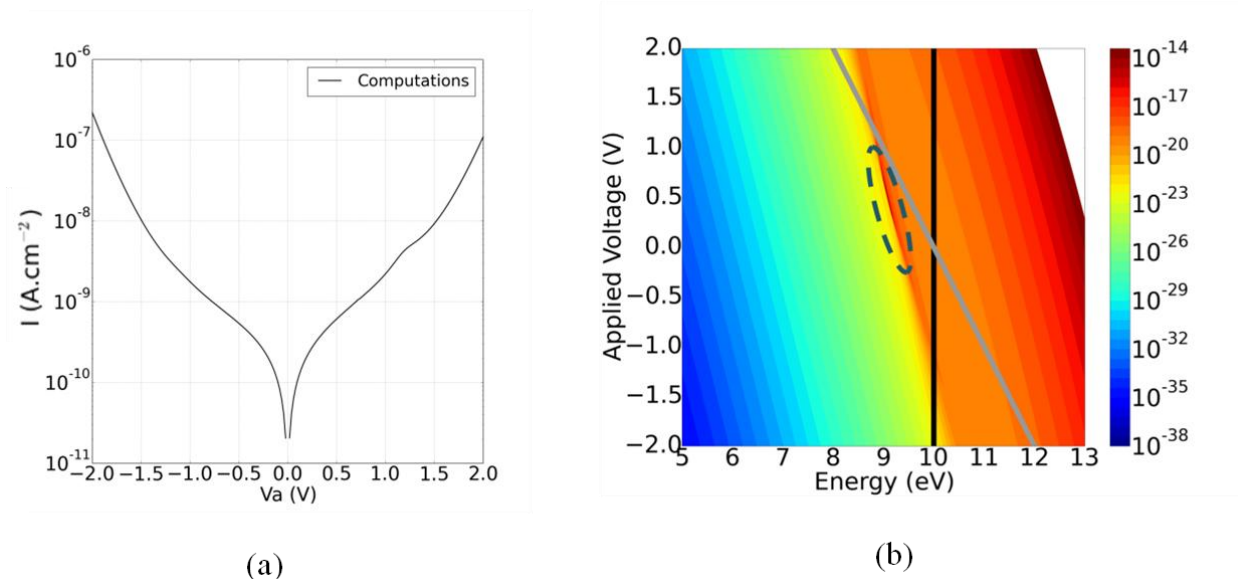
FIG.8. Computed (a) I(V_a) characteristics and (b) color map of the tunneling probability of a \text{HSC}_6\text{FcC}_7 based diode.
