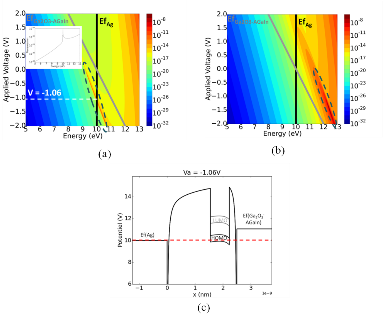
FIG. 3. The figures (a) and (b) present computed color maps of the tunneling probability for the HSC 11 FC based junction (by considering \Gamma_{\text{HOMO}} = \Gamma_{\text{LUMO}} = 0.6\text{eV} ). The computations are performed considering (a) only the HOMO and (b) only the LUMO of the ferrocenyl moiety. The resonant states are surrounded by dashed lines. (c) Potential inside the HSC 11 FC based molecular diode at V_a = -1.06 V ( \Gamma_{\text{HOMO}} = \Gamma_{\text{LUMO}} = 0.6\text{eV} ). The inset of the figure (a) shows the transmission probability versus energy for V_a = -1.06 eV.
