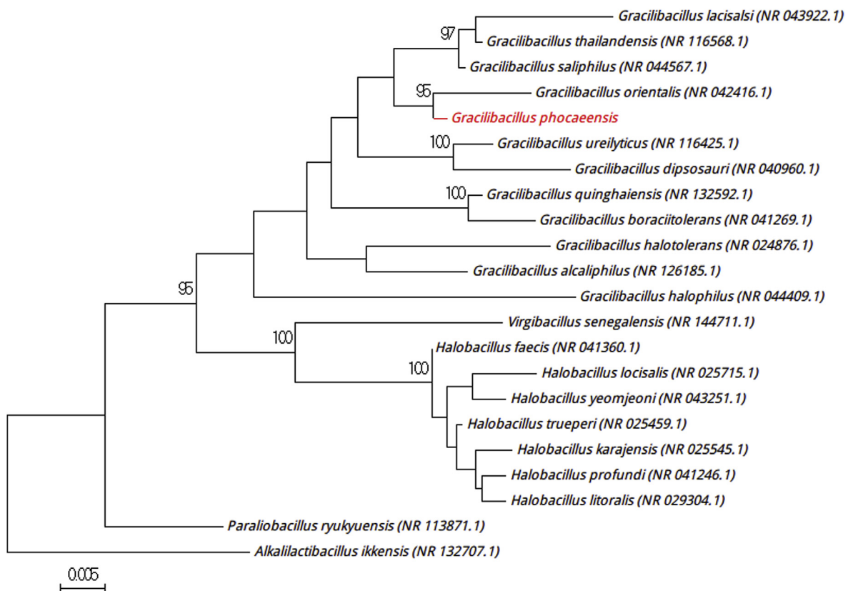
FIG. 1. Phylogenetic tree showing position of ' Gracilibacillus phocaeensis ' Marseille-P3801 T relative to other phylogenetically close neighbours. 16S rRNA gene sequences were aligned using ClustalW, and phylogenetic inferences were obtained using maximum-likelihood method within MEGA software. Numbers at nodes are percentages of bootstrap values obtained by repeating analysis 500 times to generate majority consensus tree. Only bootstrap scores of \geq 75 were retained. Scale bar indicates 0.005 nucleotide sequence divergence.
