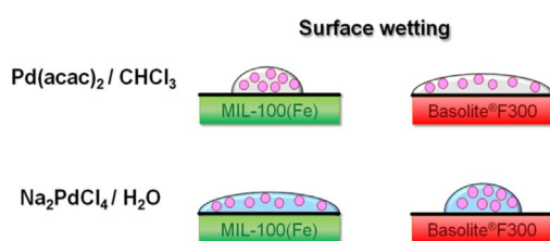
Figure 9. Surface wetting schematic of MIL-100(Fe) and Basolite® F300 when used as supports with different polar vs. apolar combinations of solvent and Pd precursor (depicted as pink circles). Pd precursor aggregates lead to larger particles upon calcination and reduction.
