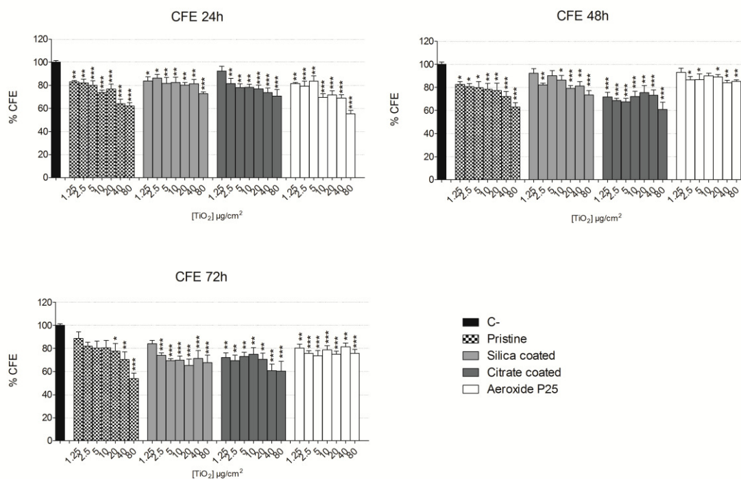
Figure 3. Cell viability in A549 cells exposed to TiO 2 NP evaluated by CFE assay. Cells were exposed to increasing concentrations (1.25–80 µg/cm 2 ) of NP for 24, 48 and 72 h. Data are plotted as mean %CFE values normalized to the untreated control (C-; black bar) ± standard error of the mean (SEM); n= 6. * P <0.05, ** P <0.01, *** P < 0.001. C+: 1000 µM Na 2 CrO 4 that induced 0% CFE (data not shown).
