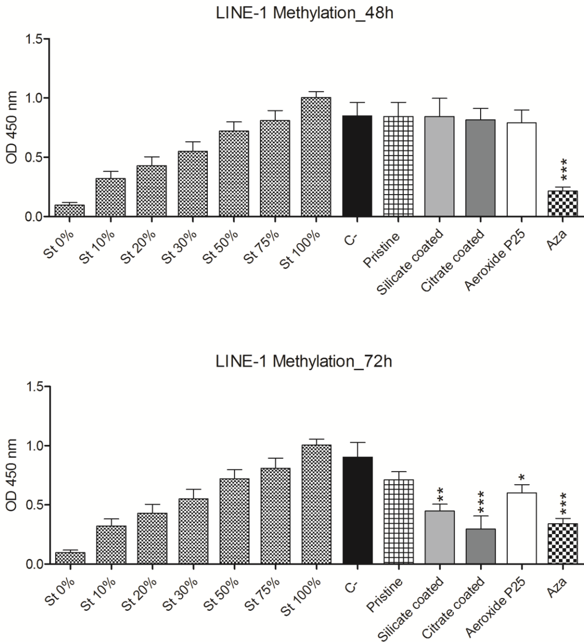
Figure 8. LINE-1 methylation levels of A549 cells after TiO 2 NP exposure. A549 cells were exposed to 40 \mu\text{g}/\text{cm}^2 of TiO 2 NP for 48 and 72 h. Each data point represents the mean \pm SEM of three independent experiments. C-: untreated control; St: DNA standard with known methylation level. Aza: 5-Azacytidine. Statistical analysis performed by one-way ANOVA and Dunnet post-test. * P < 0.05 ; ** P < 0.01 ; *** P < 0.001 .
