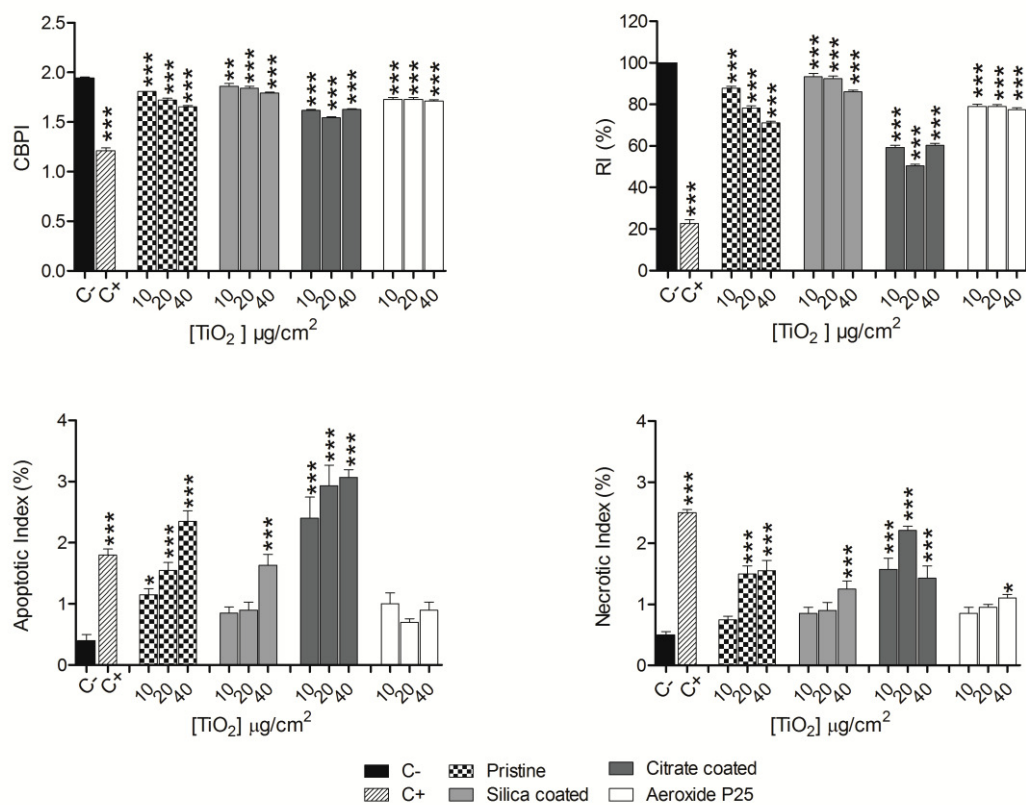
Figure 4. Cytostatic (CBPI and RI) and cytotoxic (apoptotic and necrotic index) effects induced by TiO 2 NP. Cells were exposed to increasing concentrations (10-20-40 µg/cm 2 ) of NP for 48 h. Data are plotted as mean values ± standard error of the mean (SEM); n= 4; statistical analysis performed by one-way ANOVA and Dunnet post-test.* P < 0.05, *** P < 0.001. As positive control 0.10 µg/ml mitomycin-C was employed.
