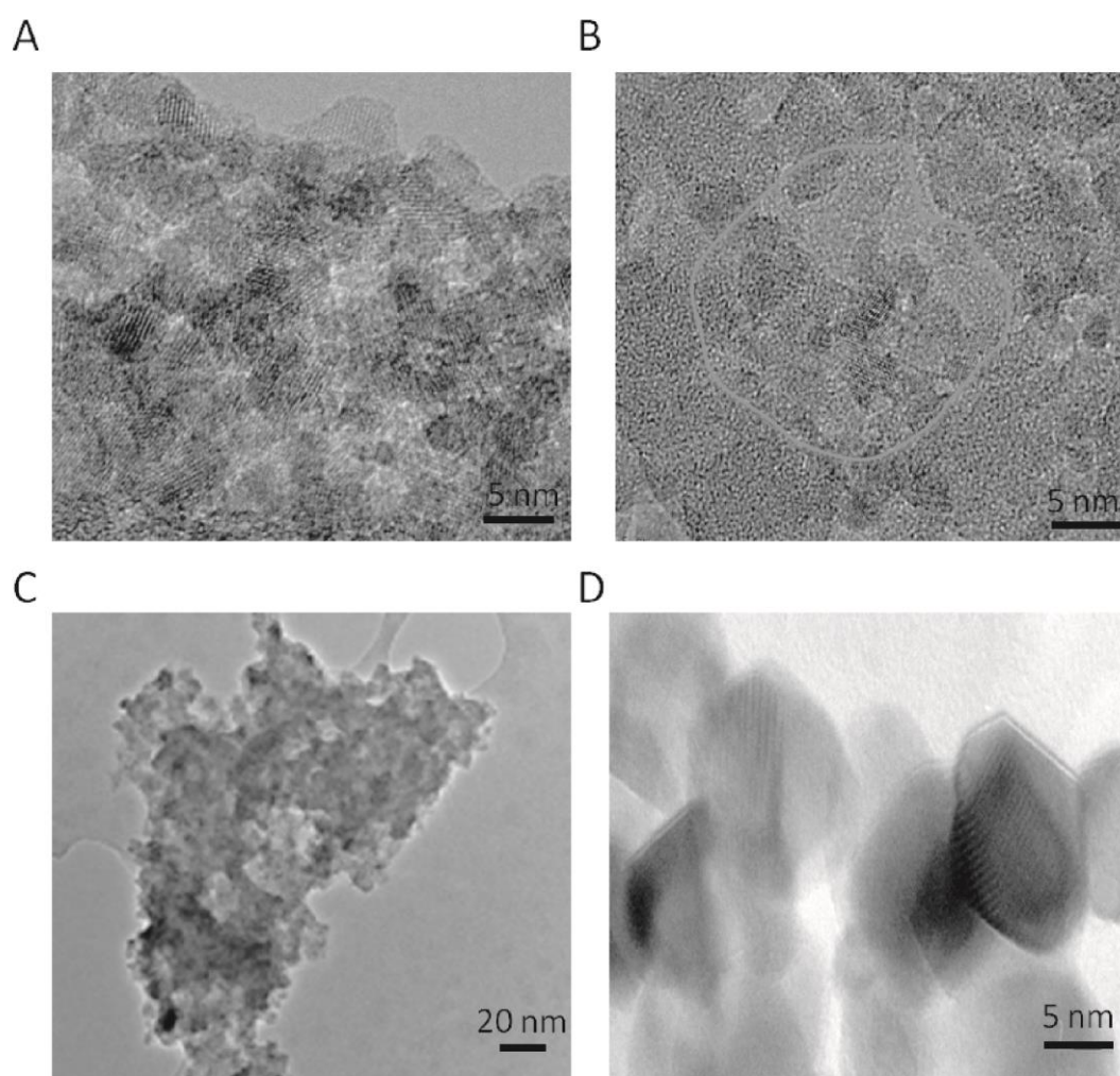
Figure 1. TEM images of TiO 2 NP. (A) pristine; (B) silica coated; (C) citrate coated; (D) P25.
