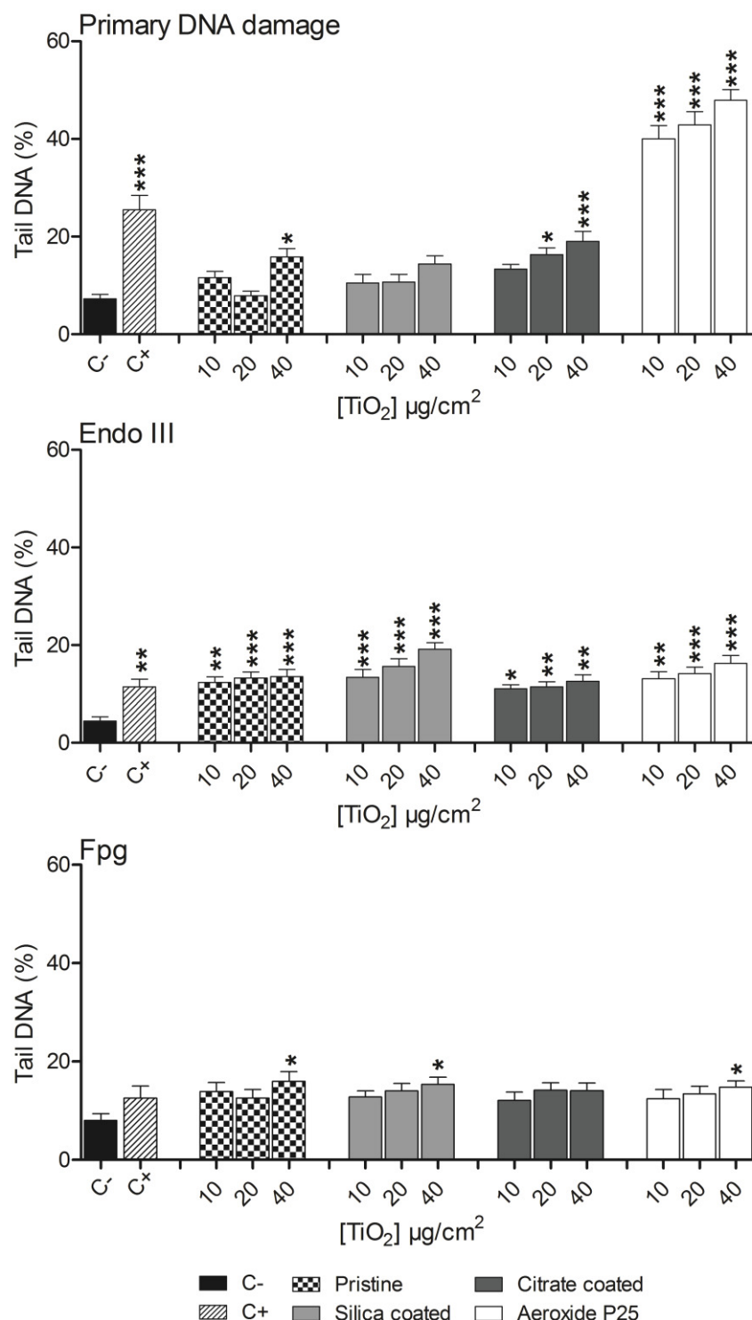
Figure 7. Primary and oxidised DNA lesions induced by TiO 2 NP in A549 cells treated for 48 h. The level of enzyme-sensitive sites was obtained by subtracting the value of % of DNA fluorescence in tail obtained after digestion with each enzyme and with the buffer only. Each data point represents the mean \pm SEM of three independent experiments. C+: positive control (50 \mu M H 2 O 2 ); C-: untreated control. Statistical analysis performed by one-way ANOVA and Dunnet post-test. * P < 0.05 ; ** P < 0.01 ; *** P < 0.001 .
