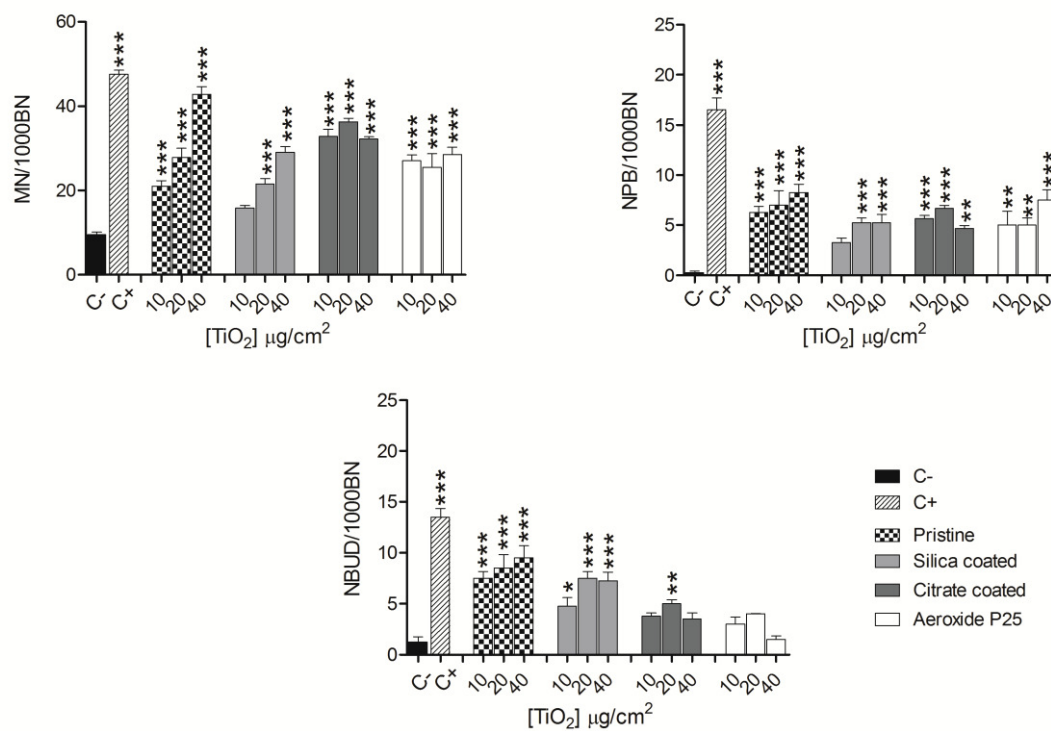
Figure 5. Chromosomal damage induced by TiO 2 NP. A549 cells were exposed to increasing concentrations (10-20-40 µg/cm 2 ) of NP for 48 h and MN, NPB and NBUD were manually scored using an inverted microscope (400X magnification). Data are plotted as mean values ± SEM; n = 4; statistical analysis performed by one-way ANOVA and Dunnet post-test. * P <0.05, ** P <0.01, *** P <0.001. As positive control 0.10 µg/ml mitomycin-C was employed.
