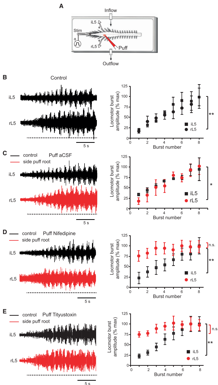
Figure 7. Slow Inactivation of Kv1.2 Potassium Channels for Powering Up Fictive Locomotor Outputs
