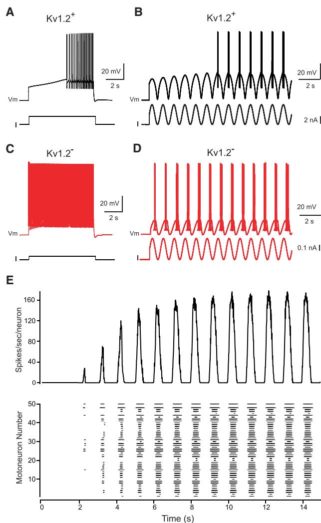
Figure 6. Firing Responses of Simulated Motoneurons to Steady and Oscillatory Depolarizing Inputs Suggest Essential Role of the Slow Inactivation of Kv1.2 Channels in Powering Up Locomotor Outputs (A–D) Sequences of action potentials evoked by depolarizing current steps (A and C) or by 1-Hz sinusoidal depolarizing currents (B and D) applied at the soma in the conditions of Kv1.2 current switched “on” (A and B) and “off” (C and D). In (A), the slow inactivation time constant was adjusted to obtain a duration of the pre-firing depolarization similar to that recorded experimentally. (E) Activity of a population of 50 uncoupled simulated motoneurons receiving the same sinusoidal stimulation as in (B). Lower panel: raster plots of the spiking activity of individual cells where each horizontal line represents a neuron and each dot represents a spike. Upper panel: integrated population activity represented by the histogram of average number of spikes per second per neuron (bin width 10 ms). The motoneurons differed in the Kv1.2 current half-activation potential, which had a Gaussian distribution with mean \pm SEM of 42.6 \pm 1.6 mV corresponding to the experimental estimates. See also Figure S7.
