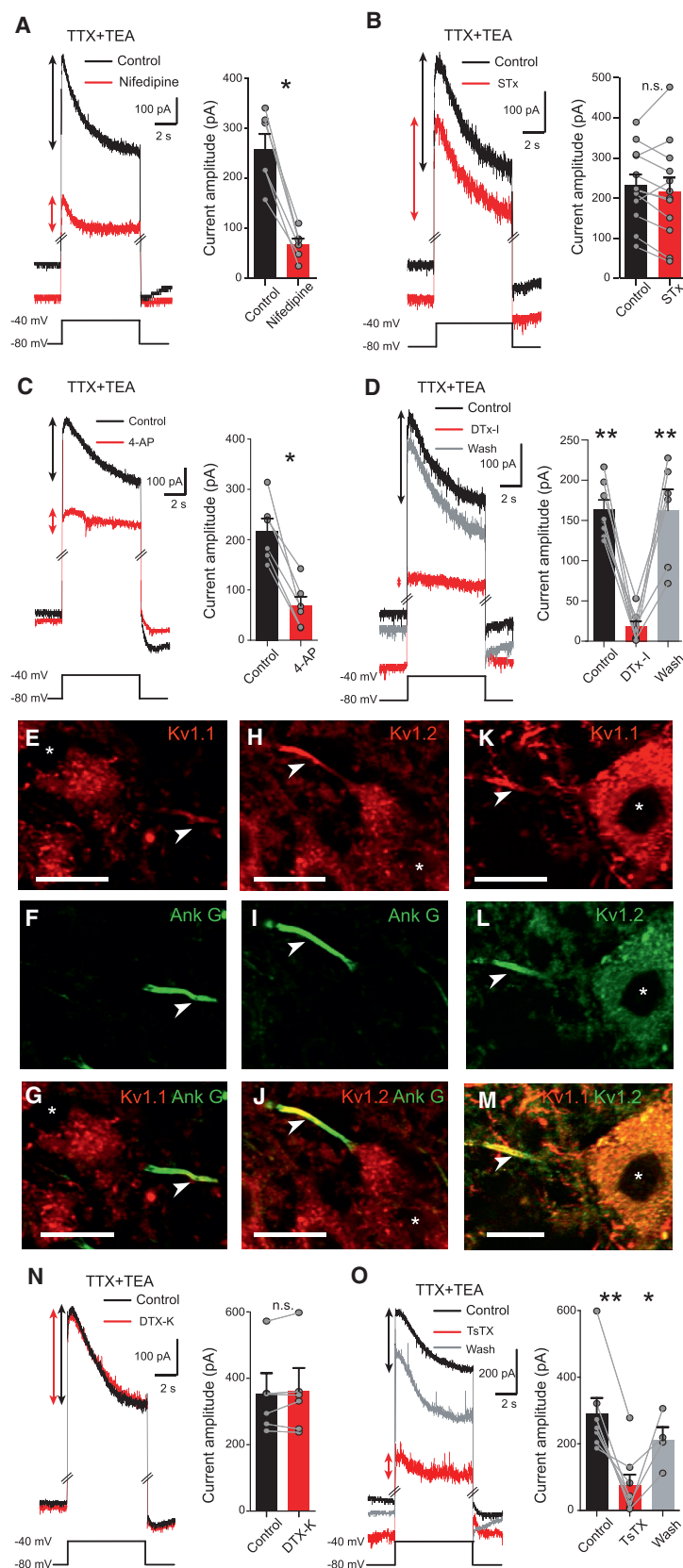
Figure 4. The Pharmacological Profile of the Outward Current Associated with Immunostaining Implicates Kv1.2 Channels
