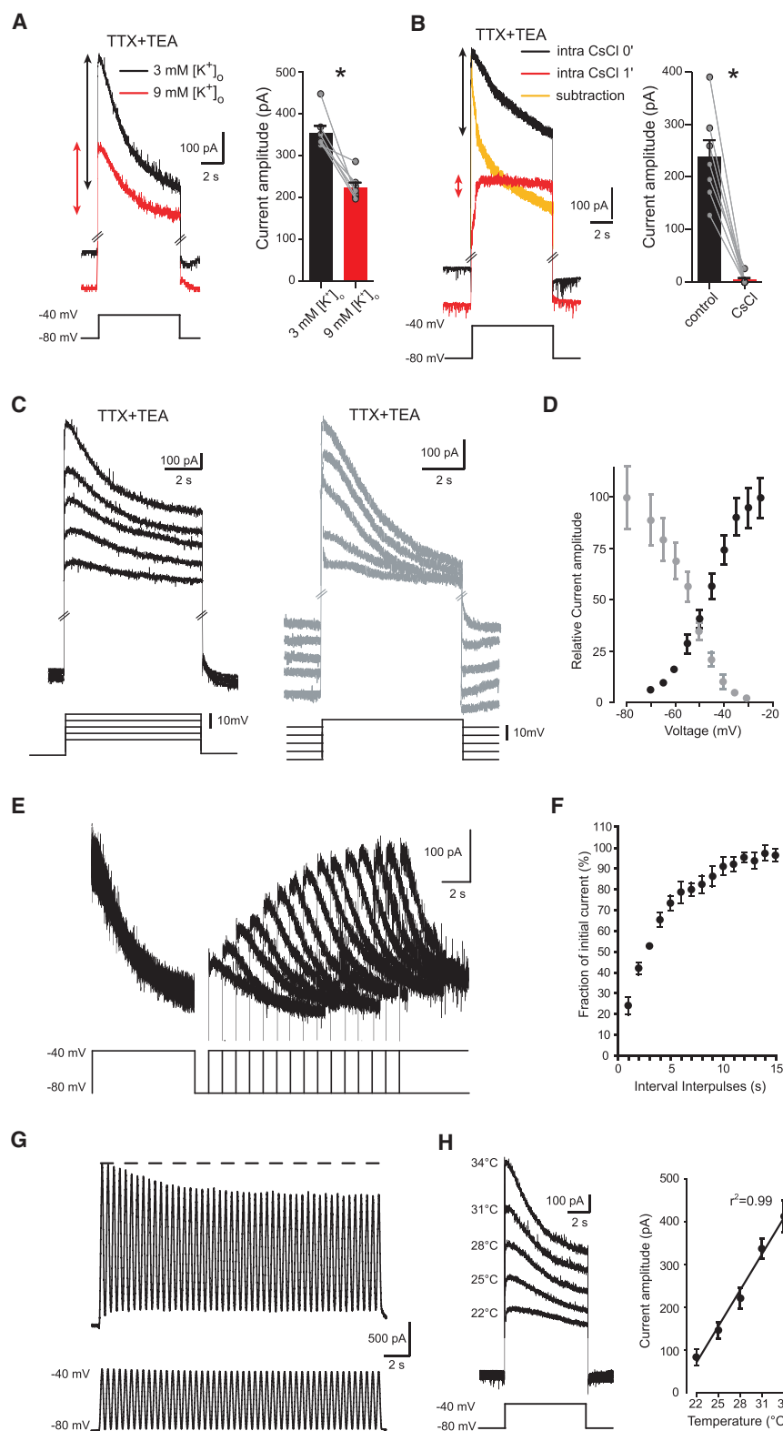
Figure 3. Biophysical Properties of Voltage-Gated K + Channel(s) Responsible for the Slow Membrane Depolarization
