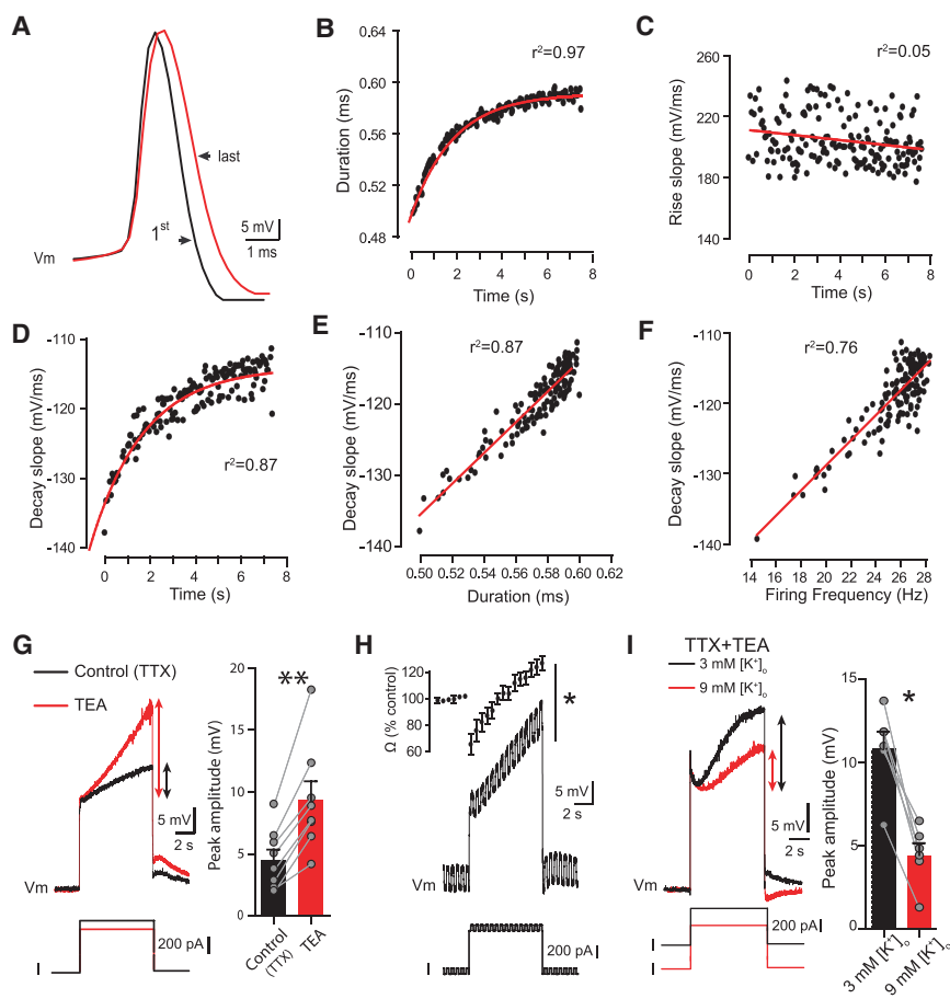
Figure 2. Slow Membrane Depolarization in Neonatal Rat Motoneurons Is Dependent on TEA-Insensitive Voltage-Gated K^+ Channels
