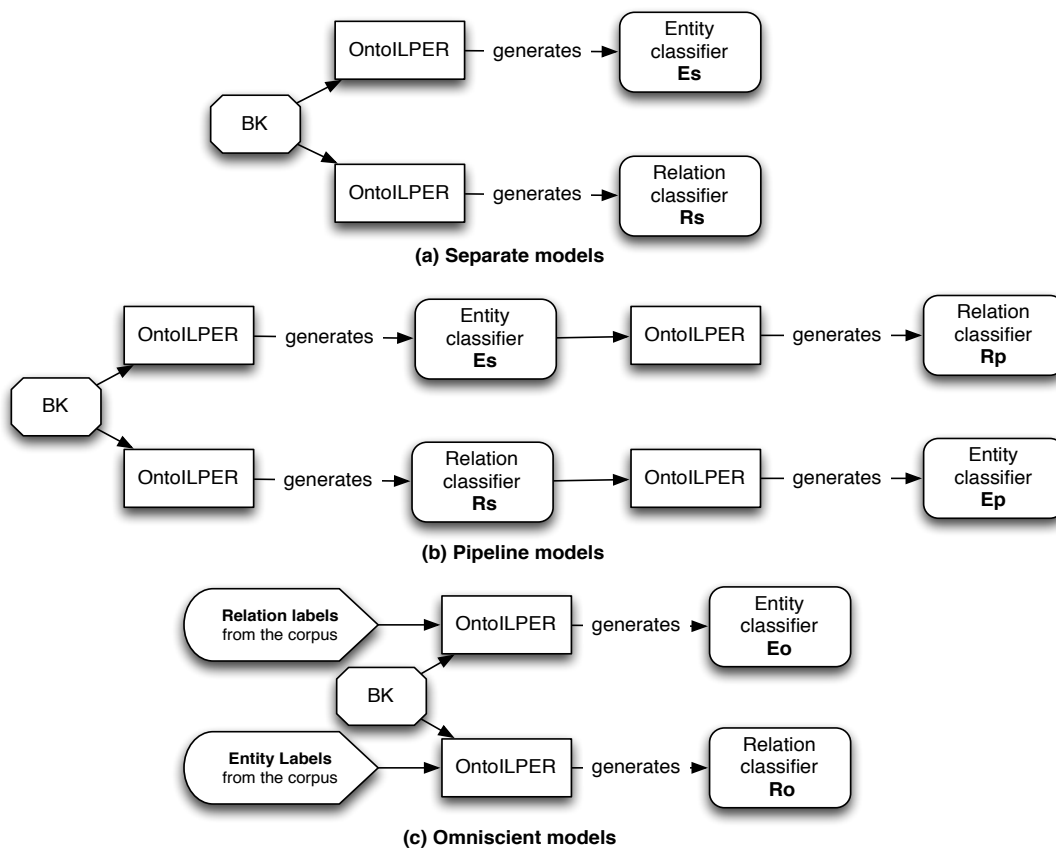
Fig. 9 Entity and relation extraction models in OntoILPER
