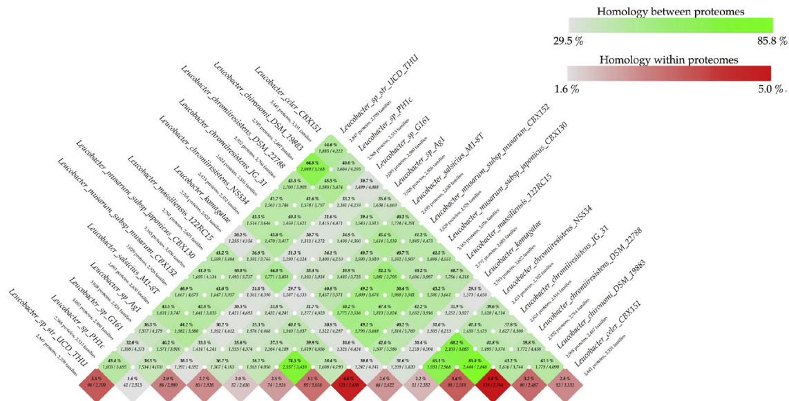
FIG. 5. A BLAST matrix of an all-against-all protein comparison of 14 Leucobacter genomes. Percentages of proteome comparisons were calculated by core genes divided by pan genes between genomes.
