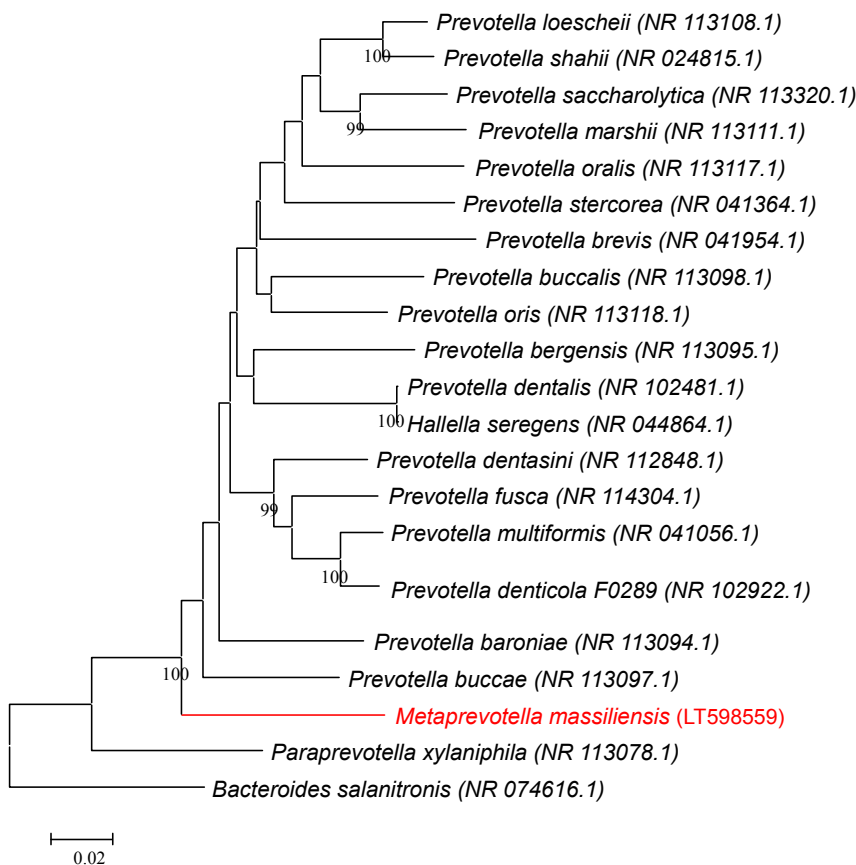
FIG. 1. Phylogenetic tree showing position of ‘ Metaprevotella massiliensis ’ strain Marseille-P-3114 T relative to other phylogenetically close neighbours. Sequences were aligned using CLUSTALW, and phylogenetic inferences were obtained using maximum-likelihood method within MEGA software. Numbers at nodes are percentages of bootstrap values obtained by repeating analysis 500 times to generate majority consensus tree. Only bootstrap scores of at least 95 were retained. Bacteroides salanitronis DSM 18170 was used as outgroup.
