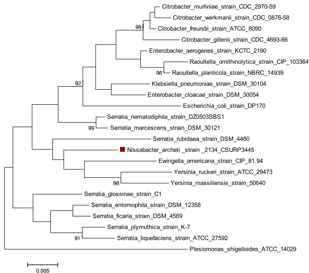
FIG. 1. Phylogenetic position of strain 2134 within Enterobacteriaceae family by 16S rDNA sequence analysis. Unrooted neighbour-joining tree of concatenated 16S rDNA of 22 reference strains of representative members of Enterobacteriaceae family closely related to strain 2134 [3]. Pleisiomonas shigelloides ATCC 14029 was used as outgroup. Values below lines are bootstrap values (1000 replicates) expressed in percent (only values greater than 90% are shown) [4]. Scale bar = accumulated changes per nucleotide. Analyses were conducted in MEGA7 [5].
