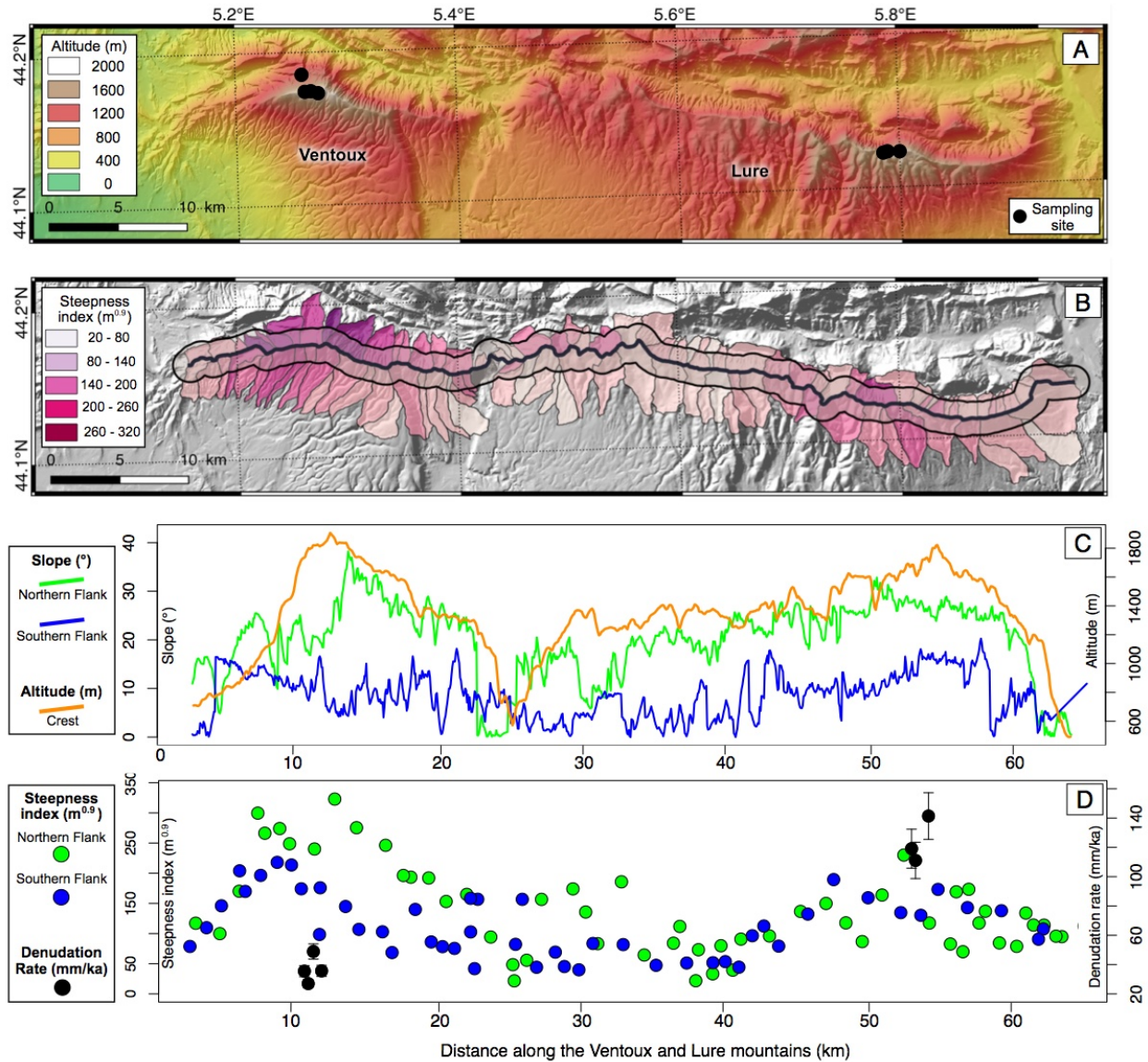
Figure 8 – A) Topographic map of the Ventoux-Lure range displaying the location of samples collected for denudation rates determination (black circles). B) Shaded-relief map showing the Ventoux-Lure crest and a 1.2 km wide buffer zone for calculation of the average slope of the flanks. Steepness indexes of selected basins ( k_{sn} ) are also displayed, with on average higher k_{sn} on the Ventoux to the West than on the Lure to the East. C) East-West profile along the Ventoux-Lure axis showing the evolution of the crest elevation (orange) and the average slopes of the northern (green) and southern (blue) flanks (see inset B for the extent of the buffer zone
