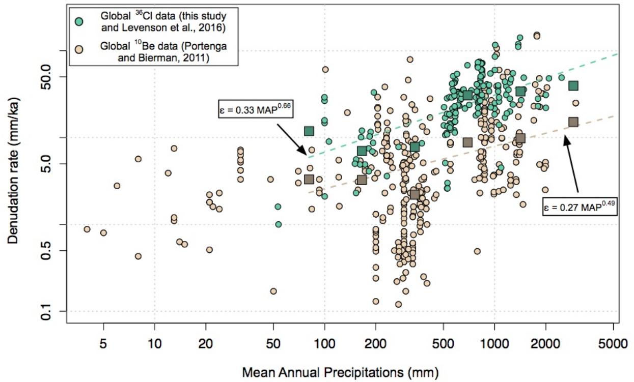
Figure 11 – ^{36}\text{Cl} carbonate denudation rates from this study and Levenson et al. (2016) compilation compared with global bedrock ^{10}\text{Be} denudation rates compiled by Portenga et al. (2011).
