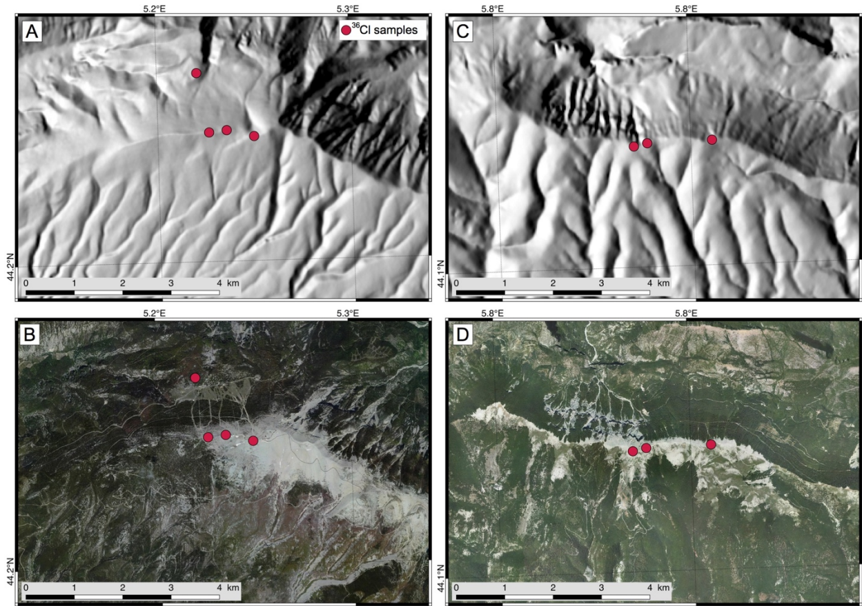
Figure 9 - A) Shaded relief map (25 m IGN DEM) centered on the Ventoux summit area. B) Corresponding orthophotography. C) Shaded relief map (5 m IGN DEM) centered on the Lure mountain summit area showing the greater development of regressive erosion and gullying on the flanks compared to the Ventoux summit. D) Corresponding orthophotography.
