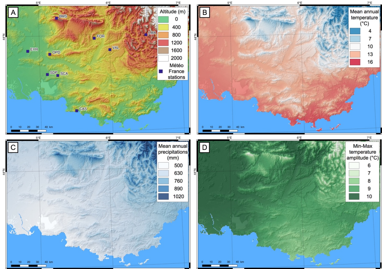
Figure 4 – A) Topographic map of Provence displaying the location of Météo France weather stations used in this work to calibrate WorldClim gridded (1 km resolution) climatic data (Fick and Hijmans, 2017). B) Mean Annual Temperatures (MAT, in °C) map of Provence, based on worldclim data. C) Mean Annual Precipitations (MAP, in mm, same source). D) Amplitude between mean annual minimum and mean annual maximum temperature (°C, same source).
