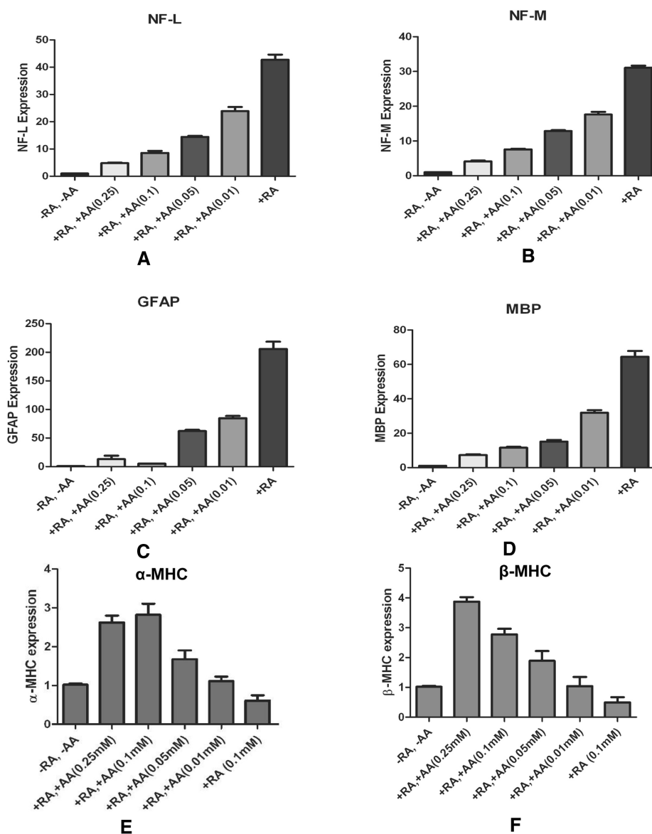
Figure 6. ES cells were incubated with RA (10 \mu M) and with increasing doses of AA. Expression of neuronal (NF-L and M, A, B ), glial (GFAP, MBP, C, D ) and cardiac muscle markers ( \alpha and \beta MHC, E, F ) was evaluated using qPCR.
