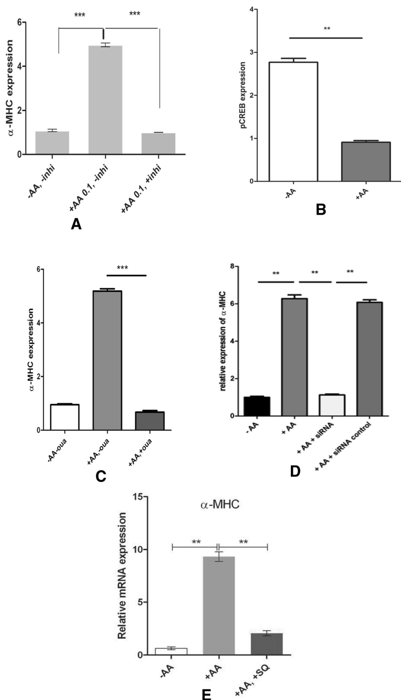
Figure 4. A. ES cells incubated or not with AA were treated with or without a p38 MAP kinase inhibitor (SB 203380) for 10 days. Cells were lysed and RNAs were extracted. Expression of cardiac \alpha -MHC was evaluated using qPCR. B. In an independent experiment, ES cells were lysed at the end of the protocol before Western blotting. Phosphorylated CREB expression was analyzed using an antibody recognizing the phosphorylated form of this protein. Western blots were scanned and band intensity was evaluated using imageJ. C. ES cells incubated with or without AA were treated with ouabain. Cardiac \alpha -MHC expression was evaluated using qPCR. D. ES cells were transfected or not with a SVCT2-specific siRNA or with a negative control siRNA (see Methods). Expression of cardiac \alpha -MHC was evaluated using qPCR. E. ES cells cultured with or without AA were treated with an adenylate cyclase inhibitor (SQ22536). Expression of \alpha -MHC was evaluated using qPCR.
