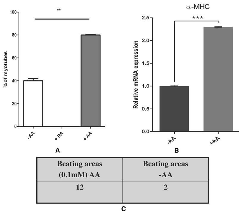
Figure 2. ES cells (CGR8) were incubated with either retinoic acid (RA) or ascorbic acid (AA) at D0 and for 10 days. A. Cells were stained with an anti-MHC antibody (see Methods) and percentage of positive cells was evaluated. B. Expression of cardiac \alpha -MHC in ES cells treated or not with AA (0.1 mM) was evaluated using qPCR. C. Evaluation of areas presenting beating cells (10 000 plated cells).
