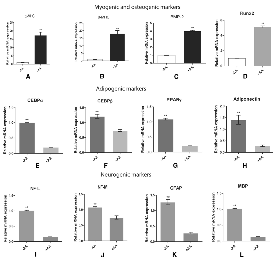
Figure 3. ES cells (CGR8) were incubated with or without ascorbic acid (AA) for 10 days, without LIF. After extraction of RNAs, we evaluated relative expression of specific markers: muscle MHC (A and B) as markers of myogenesis, BMP and Runx2 (C and D) as markers of osteogenesis, CEBP \alpha and \beta (E, F), PPAR- \gamma (G) and adiponectin (H) as markers of adipogenesis, NF-L and M (I, J) as neuronal markers, GFAP (K) and MBP (L) as glial markers.
