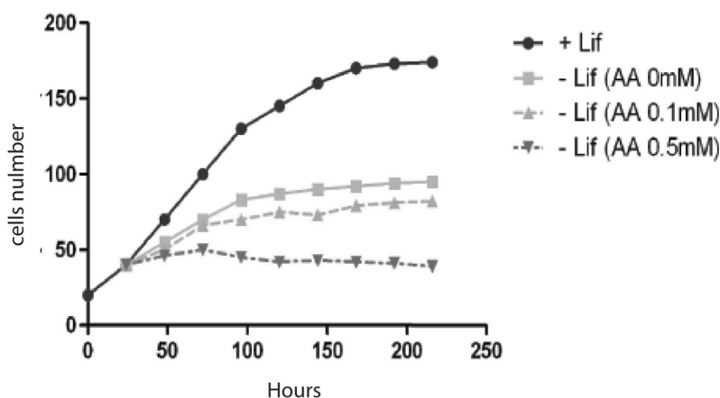
Figure 1. ES cells (CGR8) were seeded at a density of 1000 cells/cm 2 in 6-well microplates and incubated in presence or absence of AA and with or without LIF. Number of cells was evaluated from t0 to 220 h. Y-axis plots cell number \times 10^{-2} .
