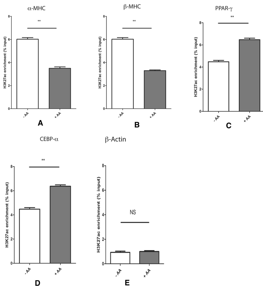
Figure 8. A. ES cells were incubated for 9 days with or without AA (0.1 mM). Chromatin was extracted (see Methods) and immunoprecipitated using an antibody raised against H3K27ac (see Methods). DNA was extracted and presence of the promoter of selected genes in the immunoprecipitated fraction was evaluated using genomic qPCR. Four genes were selected: \alpha MHC (A), \beta MHC (B), PPAR \gamma (C), CEBP \alpha (D). Promotor of cytoplasmic actin was also evaluated as a control (E). Results are expressed as ‘% of input’ in the ChIP fraction.
