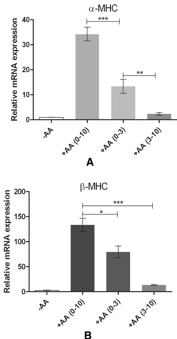
Figure 5. ES cells were treated with AA from day 0 to day 10, from day 0 to day 3 or from day 3 to day 10. RNAs were extracted. \alpha and \beta -cardiac MHC was evaluated using qPCR.
