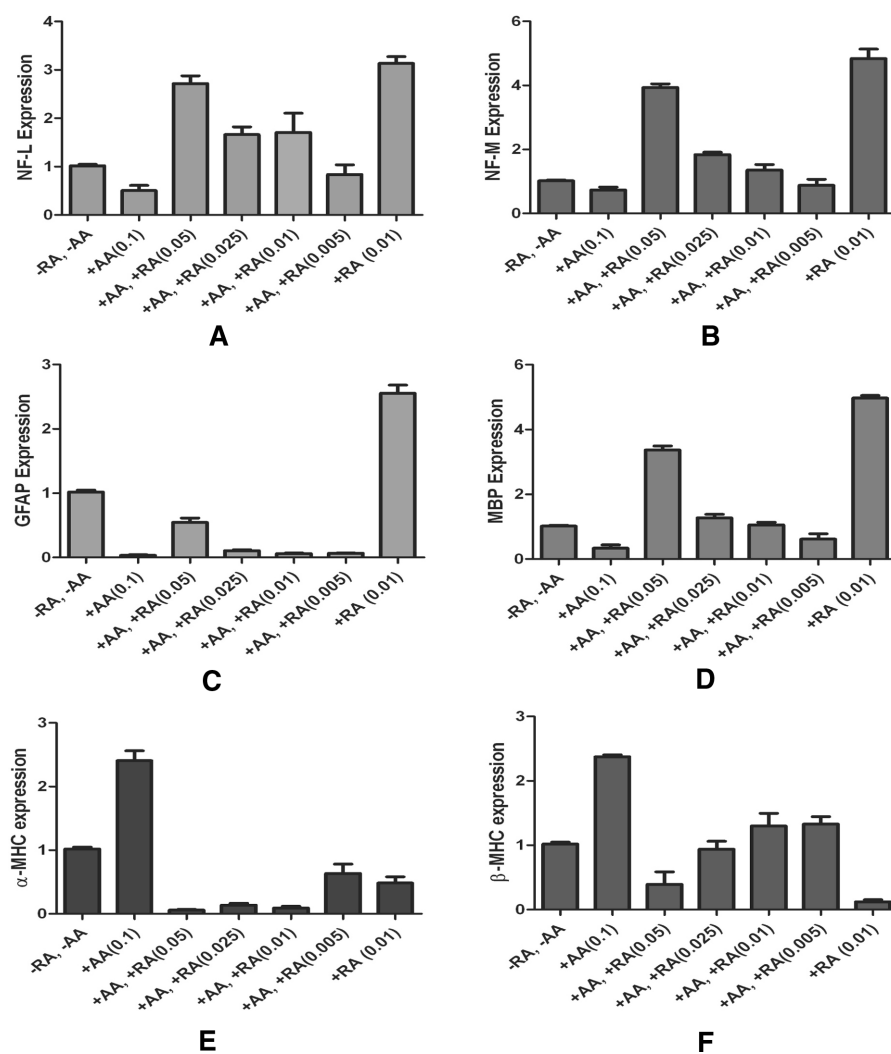
Figure 7. ES cells were incubated with AA (0.1 mM) and with increasing doses of RA. Expression of neuronal (NF-L and M, A, B ), glial (GFAP, MBP, C, D ), and cardiac muscle markers ( \alpha and \beta MHC, E, F ) was evaluated using qPCR.
