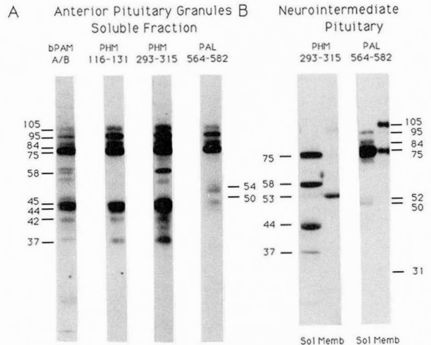
Fig.8. Western blot analysis of soluble and particulate fractions. The same preparation of anterior pituitary secretory granules analyzed in Fig.6 was frozen, diluted with an equal volume of water and granule membranes were removed by ultracentrifugation. Proteins in the soluble fraction
