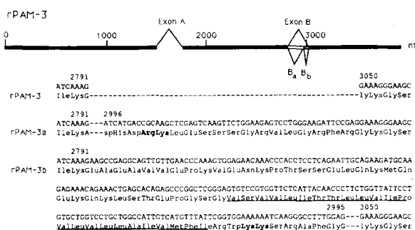
FIG. 2. Alternative splicing in the exon B region: rPAM-3a and -3b. The nucleotide and amino acid sequences of rPAM-3a and -3b in the region previously referred to as exon B are shown; the remainder of the sequence is identical to that of rPAM-2 (16, 18). Paired basic amino acids are boldface ; amino acids in the putative transmembrane domain are underlined .
