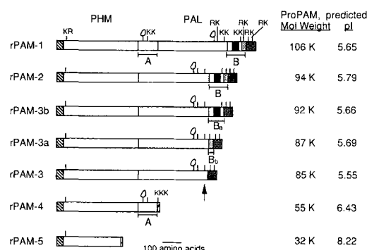
FIG. 9. PAM proteins. The proteins encoded by each type of PAM mRNA are drawn to scale with the signal peptide (cross-hatched), putative transmembrane domain (filled box), exon B a (lightly stippled), remainder of the COOH-terminal domain (darkly stippled), and potential paired basic amino acid endoproteolytic cleavage sites (K = Lys, R = Arg) and N-glycosylation sites (irregular enclosed shape) indicated. Predicted molecular weights and isoelectric points (pI) of the nonglycosylated proproteins are shown. Arrows, endoproteolytic cleavage site thought to be used in the production of the 75-kDa PAM protein from rPAM-2, -3b, -3a, and -3.
