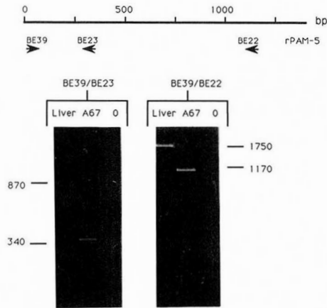
Fig.5. Structure of the PAM gene in the region preceding rPAM-5. Sprague-Dawley rat liver DNA (0.5 µg) was amplified using a sense oligonucleotide primer within the PHM domain (BE 39, bp 1172-1193 of rPAM-1) and antisense oligonucleotides from the 3'-untranslated region of rPAM-5 (BE23, bp 1496-1512, or BE 22, bp 2323-2342 of rPAM-5; numbers for rPAM-5 have been adjusted to coincide with rPAM-1). Plasmid DNA (10 pg A67) was used as a control. Amplified fragments were separated on a 1% agarose gel and the ethidium bromide stained gel is shown. Apparent molecular weights are shown to the side of each panel.
