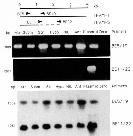
Fig. 4. Detection of rPAM-5 mRNA by RT-PCR. Reverse transcribed cDNA from the tissues indicated (Atr, atrium; Subm, submaxillary gland; Str, striatum; Hypo, hypothalamus; NIL, neurointermediate pituitary; Ant, anterior pituitary) was amplified using a pair of oligonucleotides common to rPAM-1,-2,-3,-3a,-3b and -4 (BE5/BE19) or a pair of oligonucleotides specific to rPAM-5 (BE11/BE22); extension time was 3 min and number of cycles was 30. Appropriate plasmid controls (10 pg ZAP8 for BE5/BE19 and 10 pg Ant67 for BE11/BE22) served as standards along with the blank. The same amount of input cDNA was used for both primer pairs; amounts were selected based on the prevalence of total PAM mRNA in each tissue (Braas et al., 1989). Upper. The location of the oligonucleotide primers used is indicated. Middle. Ethidium bromide stained gels. Lower. Southern blots; the 1.3 kb probe derived from the PHM domain (Fig.1) was used to detect the products amplified with BE5/19 and the 0.2 kb probe derived from Ant67 (Fig.3) was used to detect products amplified with BE11/22.
