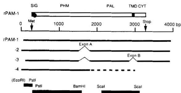
Fig. 1. PAM cDNAs identified in Adult Rat Pituitary. The structures of the 4 types of rPAM cDNA characterized from an atrial library are shown (16-18). Exons A and B are indicated, as are the rPAM-1 cDNA fragments used as probes to screen the pituitary libraries: EcoRI (cloning site used in construction of library)/PstI, bp 117-356; PstI/BamHI fragment, bp356-1682; Scal/Scal fragment, bp 2229-3190. Key features of the PAM protein are indicated for orientation: Met, Initiator methionine; SIG, signal peptide; PHM; PAL; TMD, transmembrane domain; CYT, cytoplasmic domain. Stop, termination codon.
