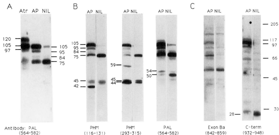
FIG. 6. Comparison of PAM proteins in atrial, anterior, and neurointermediate pituitary secretory granules by Western blot analysis. A, a crude secretory granule fraction was prepared from adult rat anterior and neurointermediate pituitary and from adult rat atrium by differential centrifugation. The atrial and anterior pituitary samples each contained 20 pmol/h PAM activity (8.4 and 19.6 \mu g of protein, respectively); the neurointermediate pituitary sample contained 4 pmol/h PAM activity (15 \mu g of protein). The samples were visualized with PAL antibody (Ab69). B and C, a more concentrated preparation of crude pituitary granules was analyzed. Each sample of anterior pituitary granules contained 100 \mu g of protein (1150 pmol/h PHM activity; 3100 pmol/h PAL activity). Each sample of neurointermediate pituitary granules contained 97 \mu g of protein (420 pmol/h PHM activity; 2900 pmol/h PAL activity). Following transfer to Immobilon-P, blots were exposed to the PAM antibodies indicated; exposure times were adjusted to give bands of comparable intensity. The exon B a antibody (Ab26) was applied to blots that had been stripped; this antibody cross-reacts with several lower molecular weight proteins not thought to be related to PAM. The location of molecular weight markers analyzed in a separate lane are indicated on the right; apparent molecular weights of the various PAM proteins are indicated on the left.
