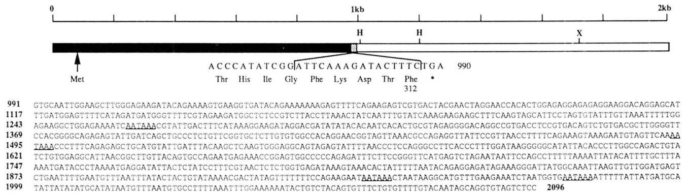
FIG. 3. Sequence of rPAM-5 type cDNA. The cDNA insert in Ant67 is drawn to scale with the region of identity to rPAM-1 shown by the filled bar and the new sequence shown by the open bar. The location of the initiator Met and the first in-frame Stop codon (*) are indicated. Characteristic restriction sites are shown: H, HindIII; X, XbaI. A cDNA probe specific for rPAM-5 was generated by using the fragment between the HindIII sites at 1001 and 1200 bp. The complete nucleotide sequence of the novel 1.1 kb 3'-region of Ant67 is shown along with the pentapeptide sequence forming the novel COOH terminus of rPAM-5; the four consensus poly(A) addition signals are underlined.
