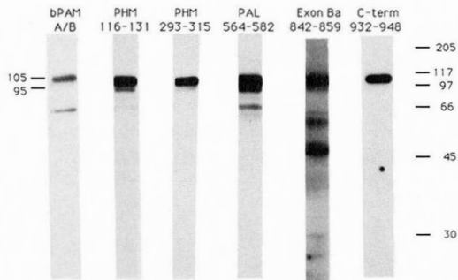
Fig.7. Western blot analysis of carbonate washed membrane fraction prepared from anterior pituitary. The crude particulate fraction from a homogenate of anterior pituitary was subjected to a series of washes with 1 M NaCl and 0.1 M Na 2 CO 3 , pH11.5 as described in Methods. Samples contained 35 µg protein and 39 pmol/h PAM activity. Antisera were used as indicated.
