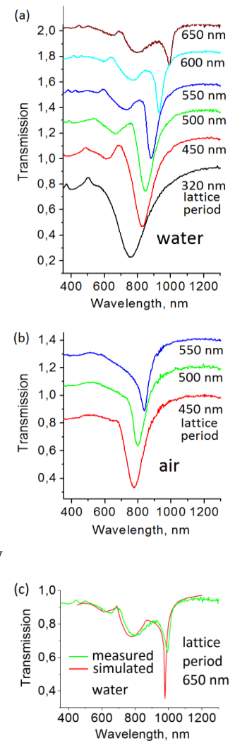
Fig.1. Measured transmission spectra of gold nanoparticle arrays with different periods of square lattice in (a) water and (b) air; (c) FDTD simulated and measured transmission spectra of 650 nm array in water.
