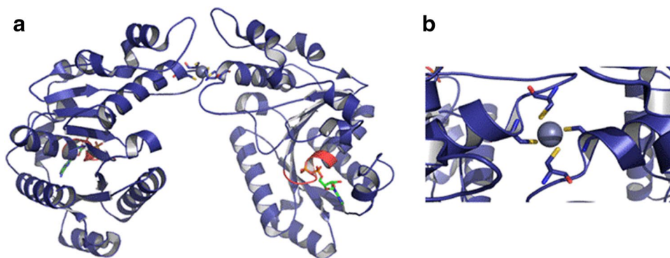
Fig. 3 a Structure of CooC-1 from Carboxydotherrmus hydrogeniformans , PDB: 3KJI [40]. b An atom of zinc in gray is at the interface of the two monomers, bound by cysteines 112 and 114. ADP is bound to the deviant Walker A motif (GKGGVGGKTT), shown in red
