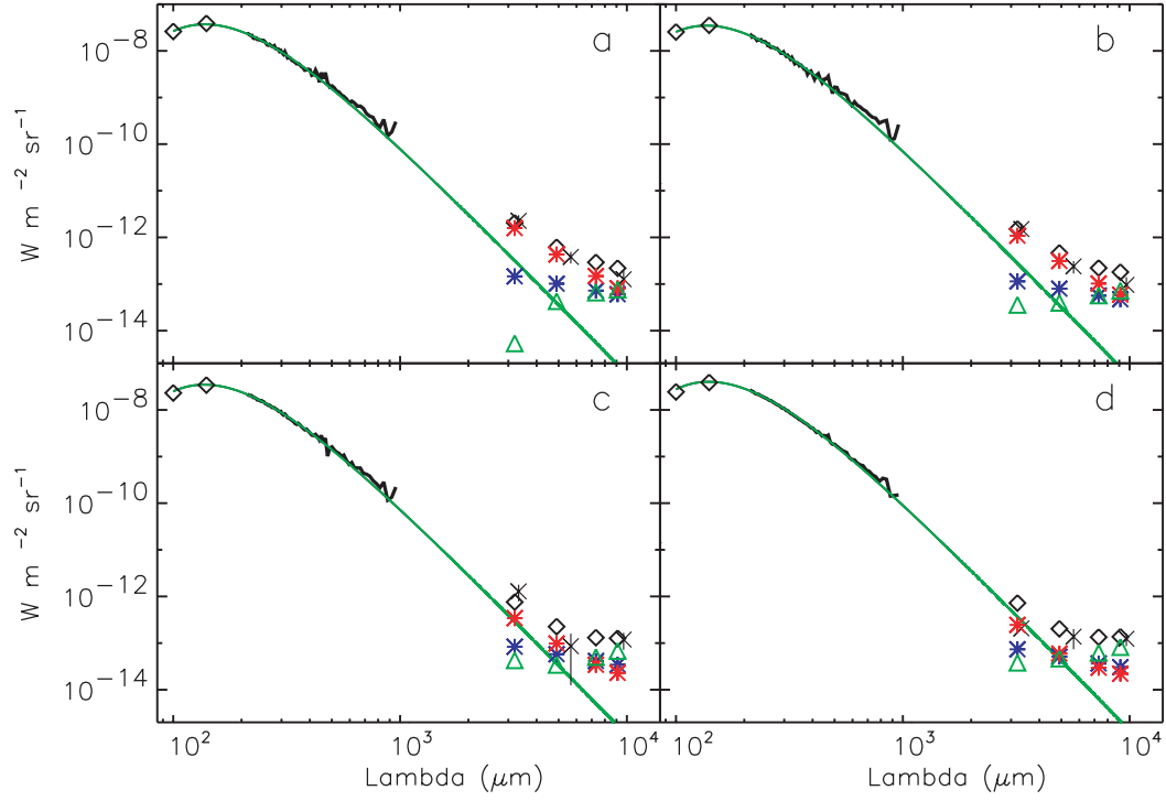
Fig. 1. Spectrum of the HI-correlated component normalised to 10^{20} at/cm ^2 (with increasing N(\text{HI}) from a ) to d ). The black diamonds at 100 and 140 \mu\text{m} are the DIRBE data, the black curve is the FIRAS spectrum, the black crosses with error bars are the DMR data and the black triangles at 3.2, 4.9, 7.3 and 9.1 mm are the WMAP data. Also displayed are the free-free and synchrotron contributions (blue stars and green triangles respectively). The green continuous line is the result of a fit of the DIRBE 100, 140 \mu\text{m} and FIRAS spectra ( 200 < \lambda < 500 \mu\text{m} ) with a modified Planck curve with a \nu^2 emissivity law (the so-called stable thermal dust component). The residual WMAP emission (which is the WMAP -free-free – synchrotron – stable thermal dust component) is shown as red stars.
