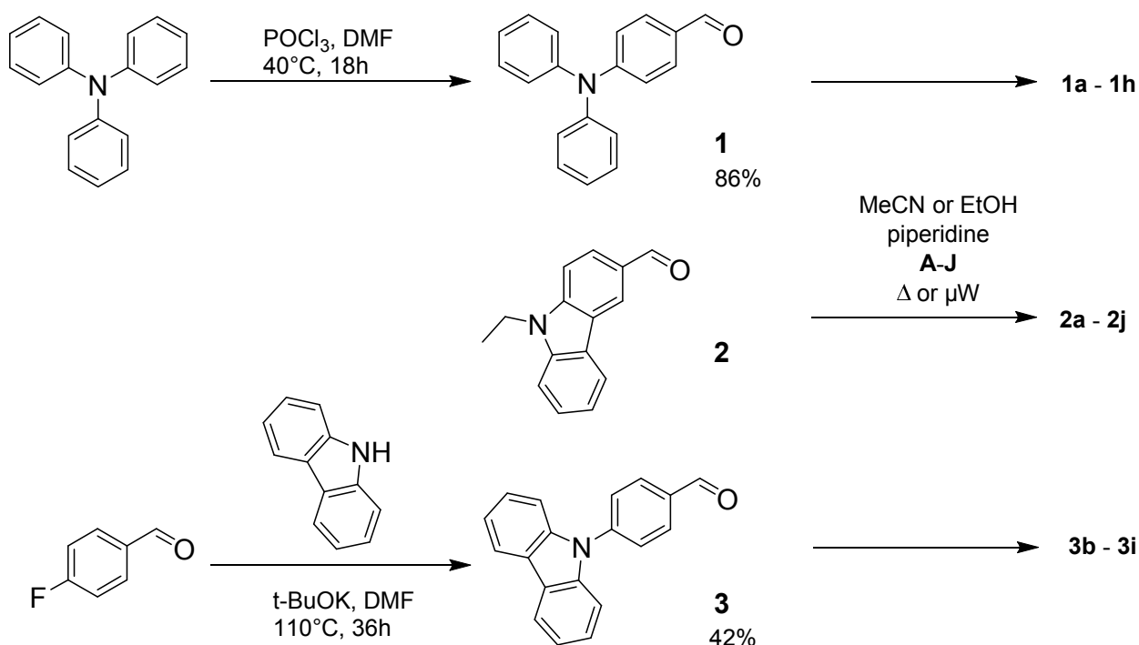
Scheme 1. Structures of activated methylene compounds A-J and synthesis of fluorophores 1a-1h , 2a-2j and 3b-3i .
