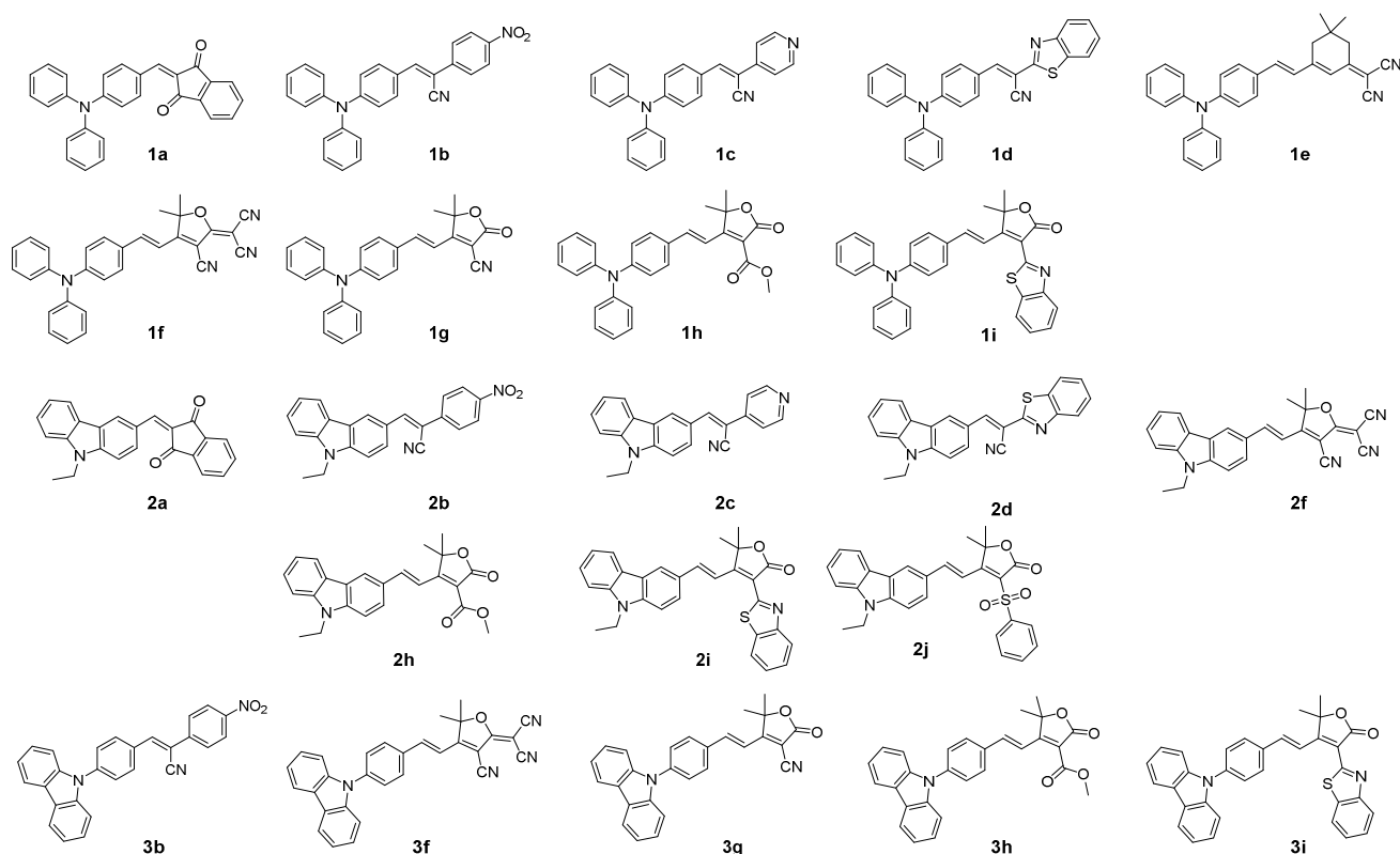
Chart 1. Structures of fluorophores 1a-1i , 2a-2j and 3b-3i .
