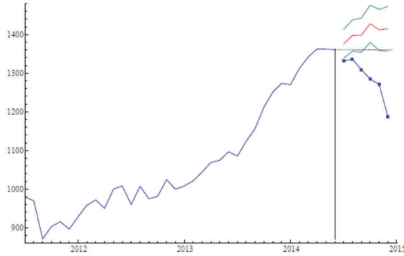
Figure 8. Unconditional forecasts for various sub-periods (with one standard error confidence intervals) – red line is the forecast and blue dots are the observed prices.
