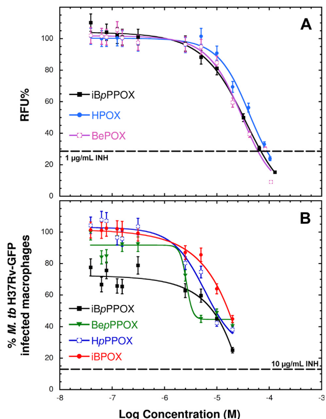
Fig. 2. In vitro and ex vivo dose-response activity of the OX derivatives against M. tb H37Rv. (A) Activity of BePOX , iBpPPOX and HPOX against GFP-expressing M. tb replicating in broth medium, expressed as normalized relative fluorescence units (RFU%). The dashed line represents the level of inhibition (~70%) reached with 1 μg/mL (=7.3 μM) INH as control. The MIC 50 of BePOX , iBpPPOX and HPOX replicating in culture broth medium were 30.8 μM, 32.0 μM and 44.6 μM, respectively. (B) Activity of iBpPPOX , BepPPOX , HpPPOX and iBPOX against M. tb replicating inside Raw264.7 macrophages. Results are expressed as the percentage of infected macrophages after 5 days post-infection. The dashed line represents the level of inhibition (~87%) reached with 10 μg/mL (=73 μM) INH as control. The MIC 50 of BepPPOX , iBpPPOX , HpPPOX and iBPOX replicating inside macrophages were 3.5 μM, 8.5 μM, 9.5 μM and 17.1 μM, respectively. Each value is the mean ± SD for a triplicated dose-response. Experiments were conducted at least twice with consistent results.
