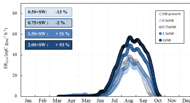
Figure 9. Sensitivity of the seasonal variation of isoprene emission rates calculated using G14 ( ER_{G14} , in \mu\text{gC}_{DM}^{-1} \text{h}^{-1} ) to SW. Overall annual relative changes to present (2000–2010) are framed.
