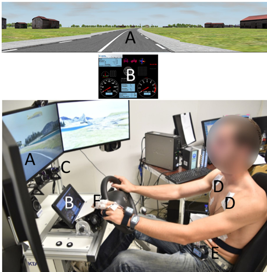
Fig. 1. The static driving simulator by Oktal®. A represents the road scene displayed on the 3 video screens. B represents the dashboard. C is the hardware faceLAB®. D are two of the three electrodes used for ECG, E is the respiratory belt. F are the electrodes for EDA (not used in this study because of important signal loss).
