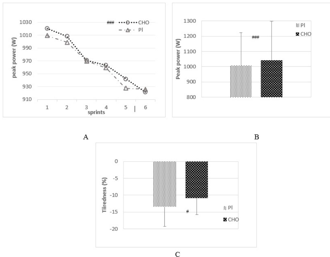
Figure 2. Evolution of peak power with sprint (A); peak power (B) and tiredness (C) with placebo (Pl) and carbohydrate (CHO) ingestion (mean \pm standard error). Notes: # when a qualitative statistics shown an effect compared with Pl condition: # likely effect, ## very likely effect and ### most likely effect.
