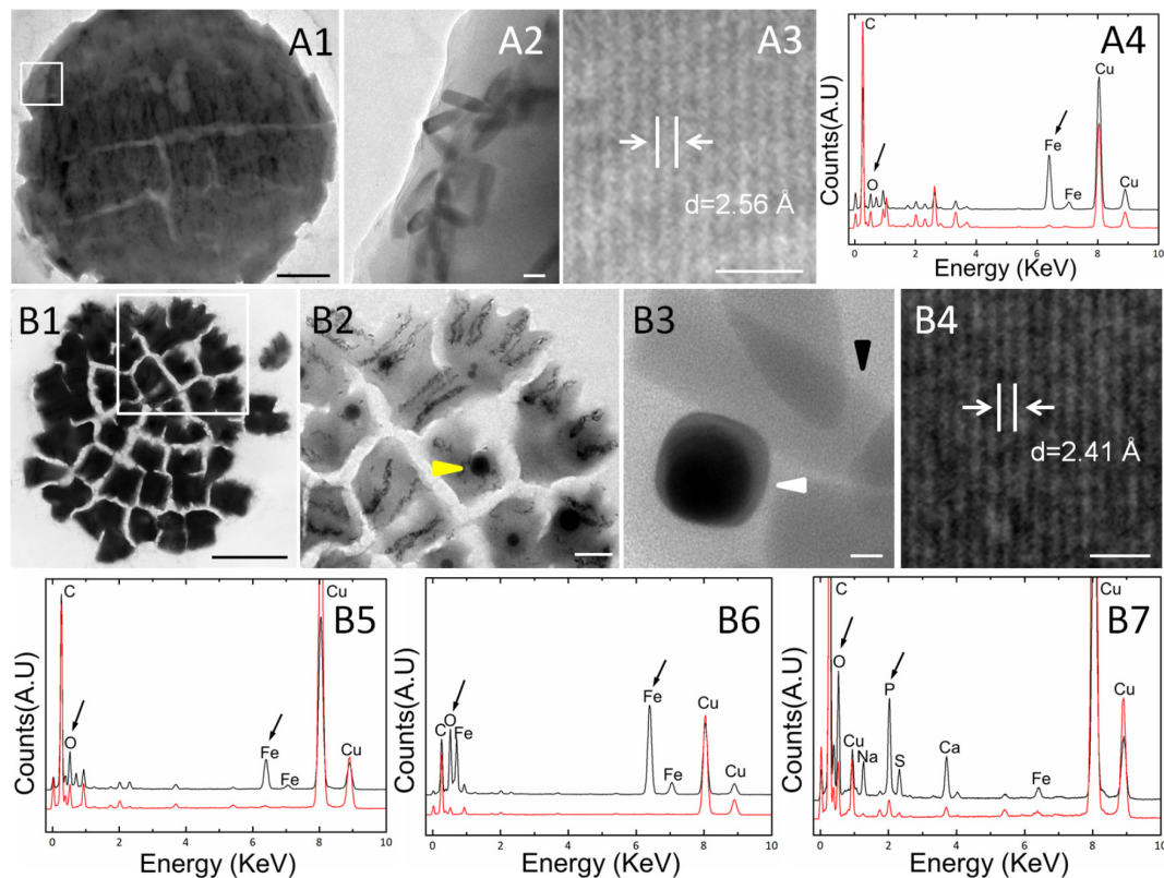
FIGURE 3 | Characteristics of magnetosomes in e-MMPs. (A) MMPs containing only bullet-shaped magnetosomes. Overall (A1) and magnified (A2) TEM views showing the bullet-shaped magnetosomes. HRTEM (A3) and EDXS (A4) spectra for the magnetite ( \text{Fe}_3\text{O}_4 ) in the bullet-shaped magnetosomes. (B) MMPs containing both bullet-shaped and rectangular magnetosomes. Overall (B1) and magnified TEM views showing inclusion bodies (B2) , yellow arrow] and bullet-shaped magnetosomes (B3) , black arrow] clustered with octahedral magnetosomes (B3) , white arrow]. HRTEM (B4) and EDXS (B5) analysis showing the spectrum of magnetite ( \text{Fe}_3\text{O}_4 ) in the bullet-shaped magnetosomes. EDXS analysis of octahedral magnetosomes (B6) and polyphosphate in the inclusions (B7) respectively. Scale bars = 2 \mu\text{m} in (A1) , 50 nm in (A2) , 1 nm in (A3, B4) , 5 \mu\text{m} in (B1) , 1 \mu\text{m} in (B2) , and 10 nm in (B3) .
