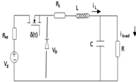
Fig. 1 DC-DC Buck Converter
