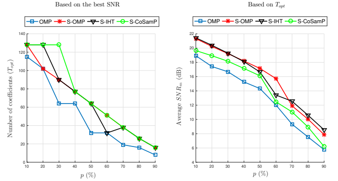
Fig. 4. Selection of T_{opt} for the sparse optimization algorithms according to the best SNR computed over the missing samples.
