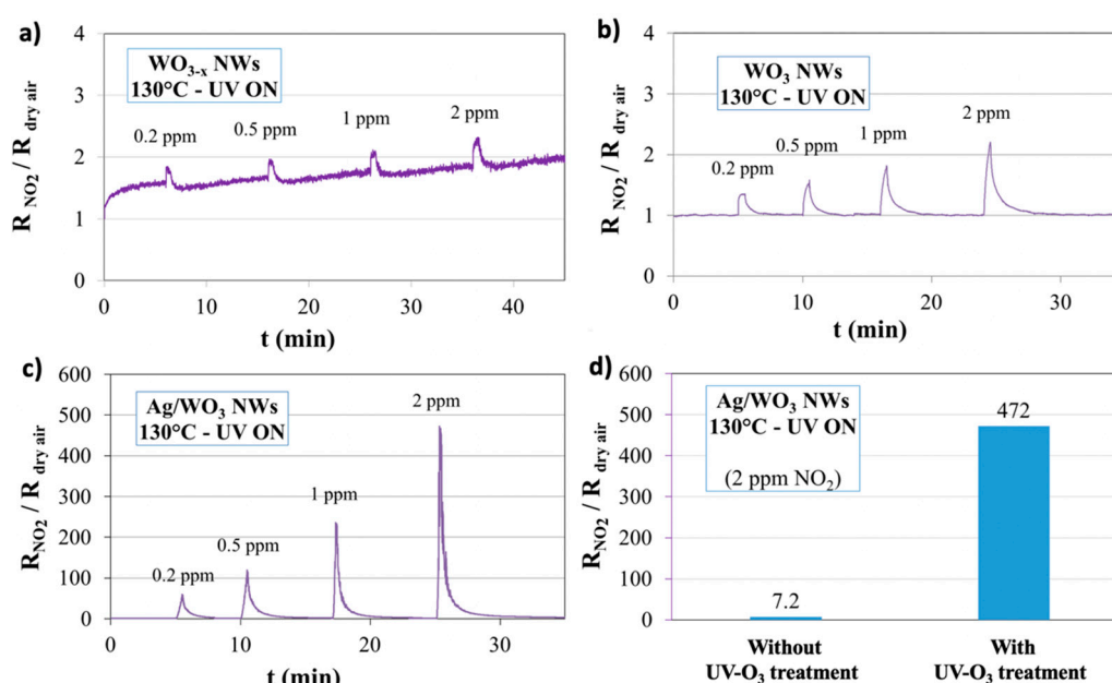
Figure 3. Sensor responses at 130 °C under UV illumination for WO_{3-x} NWs (a), WO_3 NWs (b) and Ag/WO_3 NWs (c). Comparison of the sensor responses for Ag/WO_3 NWs with or without the UV-O 3 post-treatment (d).
