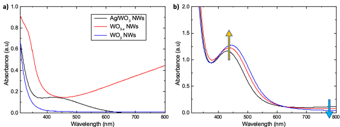
Figure 2. UV-visible absorption spectra for the three forms of tungsten oxide NWs (a) and evolution of the absorption spectra with silver growth for Ag/WO 3 NWs (b).
