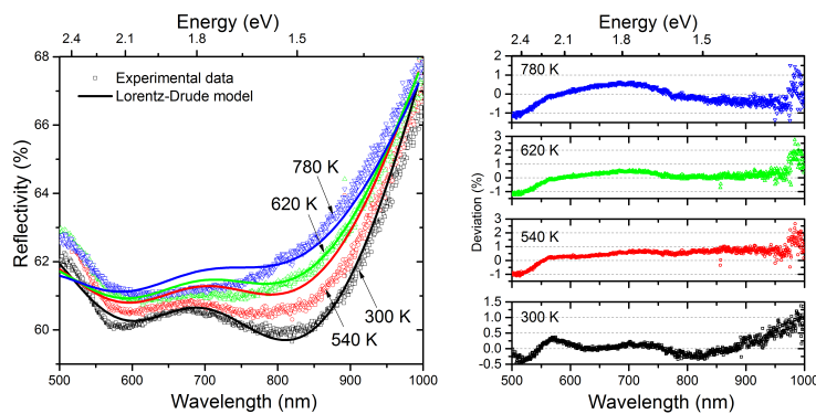
Figure 4. Left panel: measured and calculated reflectivity of unpolarized light at 20^\circ of AOI. Lines are obtained by using the Lorentz-Drude model for four different temperatures (300, 540, 620, and 780 K). Right panel: deviation between experimental and calculated reflectivity.
