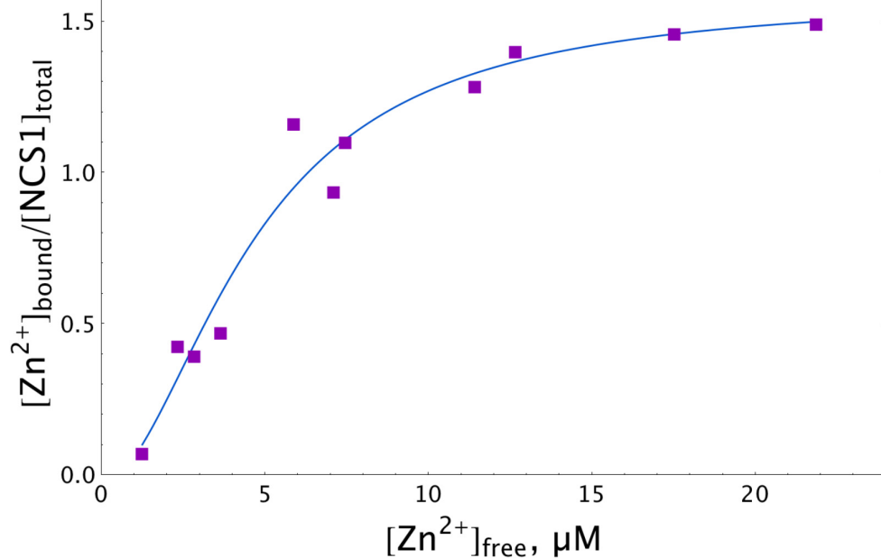
FIGURE 1 | Zn^{2+} binding to NCS-1 according to equilibrium dialysis experiments. The NCS-1 (5 \mu M) sample was pre-equilibrated with (2–150) \mu M Zn^{2+} by equilibrium dialysis (3.5 kDa MWCO) at 25°C. The concentrations of NCS-1-bound zinc ( [Zn^{2+}]_{bound} ) and free zinc ( [Zn^{2+}]_{free} ) in the resulting solutions were measured by electrothermal atomization AAS, using the absorption bands at 213.9 nm or 307.6 nm. The solid curve approximates the experimental data by Hill equation.
