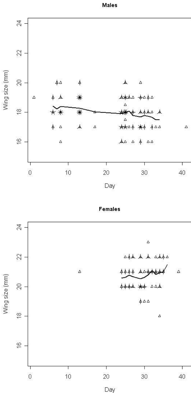
Figure 2. Forewing lengths of E. aurinia males (top) and females (bottom) captured at Deiffelt, against the days on which first captured in 1995 (Day 1 is 26 May) . Only wingwear classes 1 and 2 (out of 4) are considered. Multiple points are plotted with the numbers of radius bars corresponding to the numbers of observations. Lines depict running mean wing length for individuals captured during three consecutive trapping sessions.
