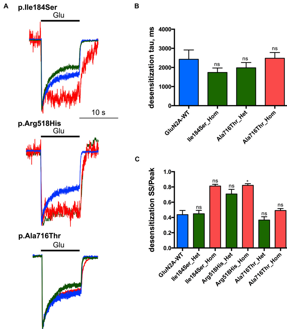
FIGURE 4 | Desensitization properties of NMDARs with mutant GluN2A subunits. Whole-cell patch clamp recordings of membrane currents were performed on HEK293T cells cotransfected with the appropriate combinations of GRIN1 and GRIN2A constructs for the expression of WT and/or of mutant recombinant NMDARs. (A) An overlay of currents evoked by 10 s Glu application in the WT (blue), homozygous (red) and heterozygous (green) conditions. Currents are normalized by peak amplitudes. (B) Averaged desensitization time constants ( \tau_{DES} ). No significant change in \tau_{DES} was detected for any condition tested. Of note, \tau_{DES} was not measurable for p.Ile184Ser in the homozygous condition, and for p.Arg518His in homozygous and heterozygous conditions because of nearly absent desensitization (Table 1). Kruskal-Wallis test with Dunn's multiple comparison test. ns: not significant. (C) Averaged steady-state to peak relation ( I_{END10s}/I_P ratio). p.Ile184Ser and p.Ala716Thr had no significant effect on I_{END10s}/I_P ratio in either of homozygous or heterozygous conditions. p.Arg518His led to significant increase I_{END10s}/I_P ratio in homozygous but not in heterozygous condition. Kruskal-Wallis test with Dunn's multiple comparison test. * p < 0.01 ; ns, not significant.
