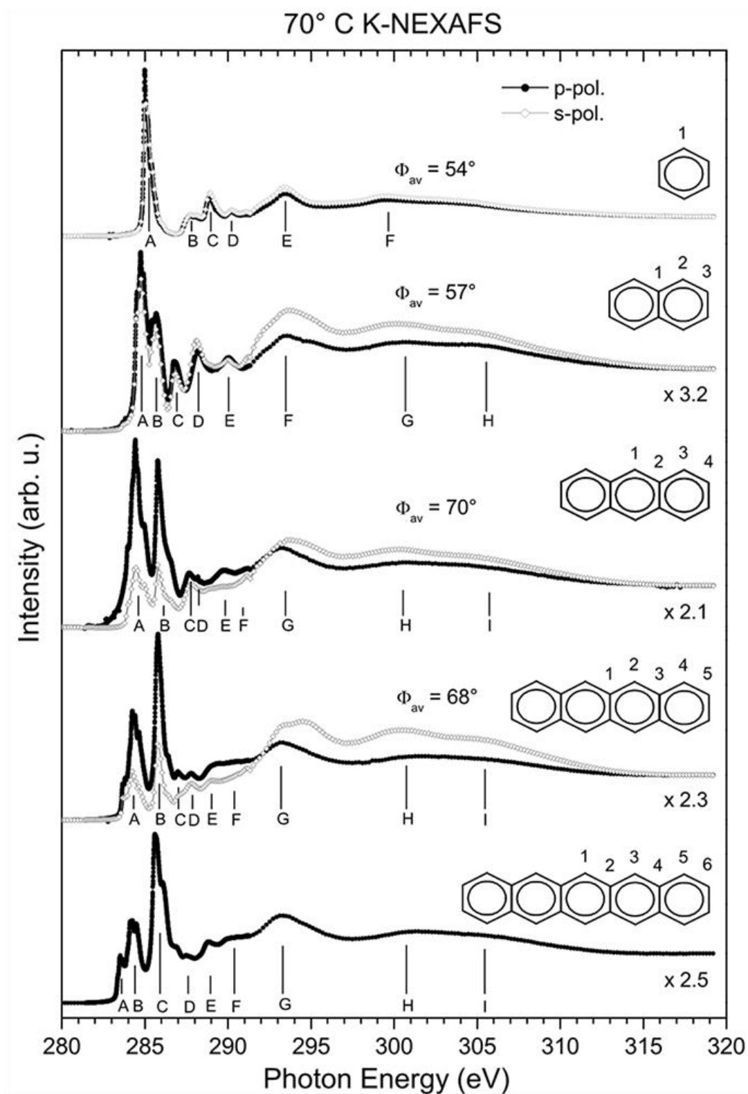
Figure 1.C K-NEXAFS of benzene, naphthalene, anthracene, tetracene, and pentacene with 70° angle of incidence from the surface normal. The average inclination angle between the molecular plane and the surface normal is obtained from the dichroism in the pre-edge. Several peaks are labeled for the discussion in the text.
