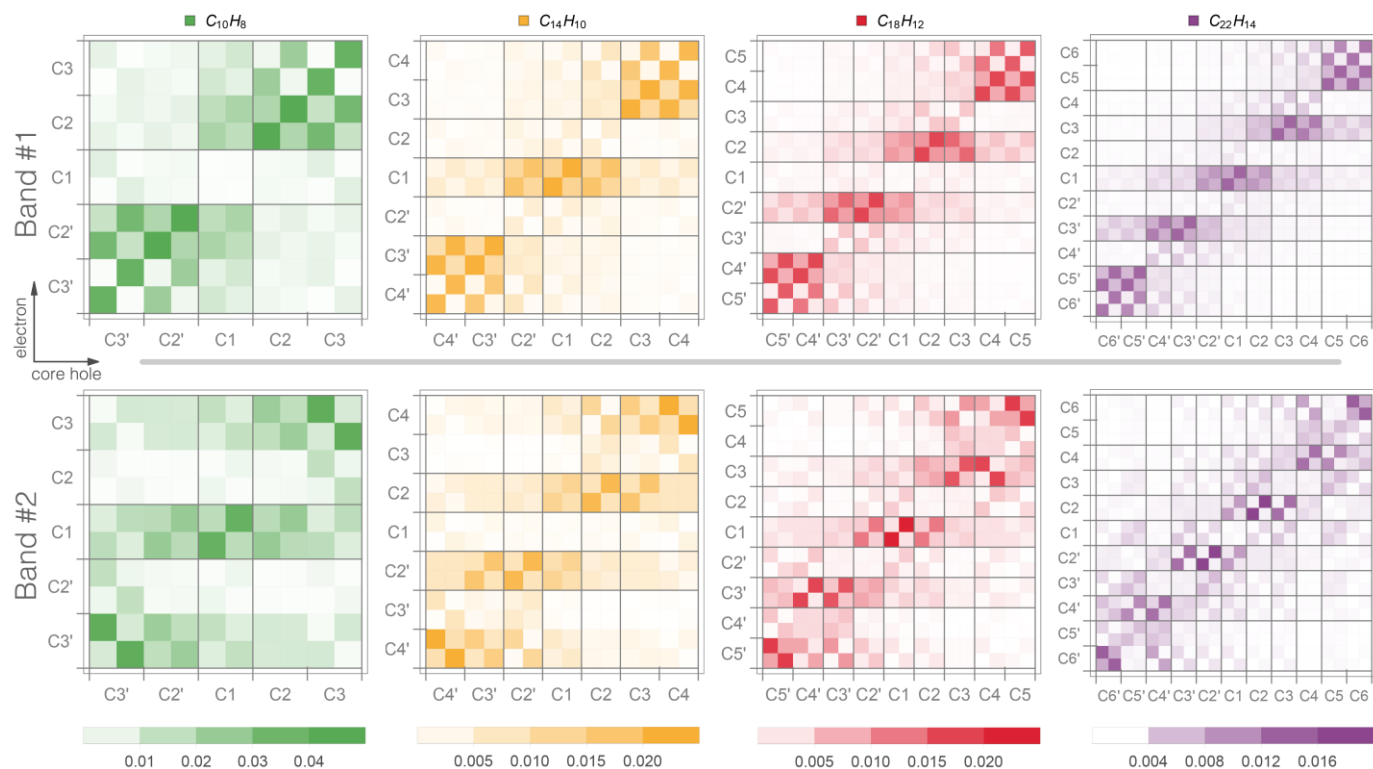
Figure 6. Electron-hole correlation plots of the combined \Omega_{AB} matrices for all carbon K-edge states in each excitation band of the electronic spectra of the polyacene molecules.
