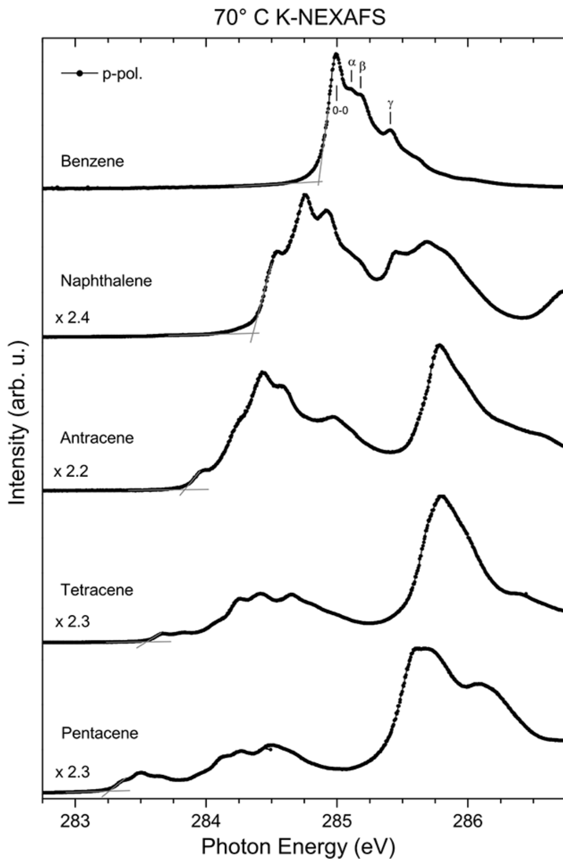
Figure 2. Blow-up of the pre-edge region of the C K-NEXAFS of benzene, naphthalene, anthracene, tetracene, and pentacene from Figure 1. The grey lines mark the NEXAFS onset.
