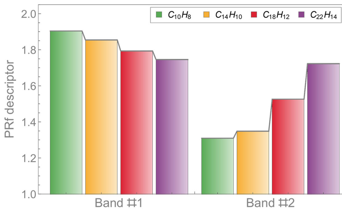
Figure 7. Mean value of the PRf descriptor for all electronic transitions of each absorption band of the spectra.
