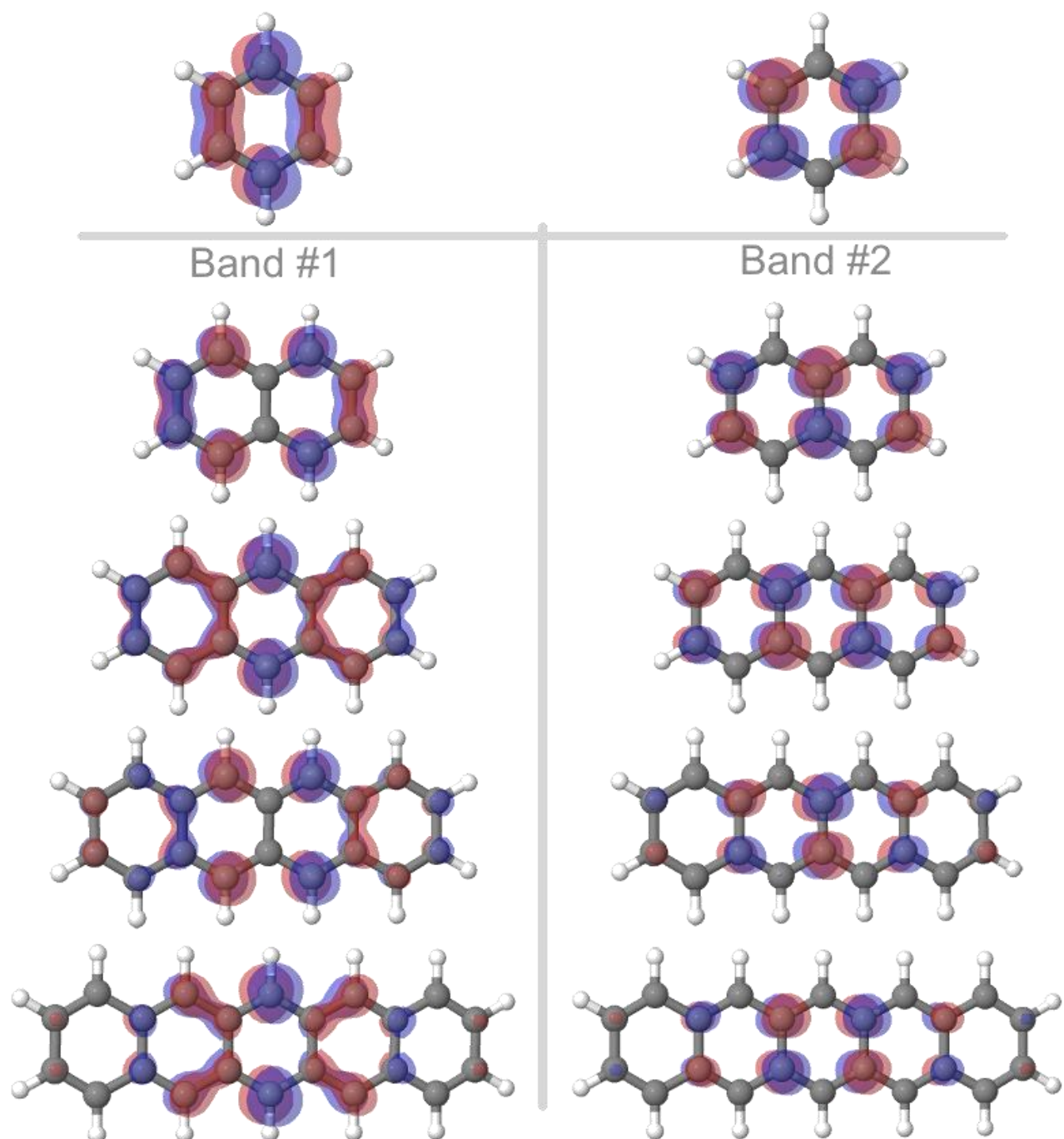
Figure 3. Natural Transition Orbitals which represent excited electrons for the most intense transitions calculated of each band of the carbon K-edge.
