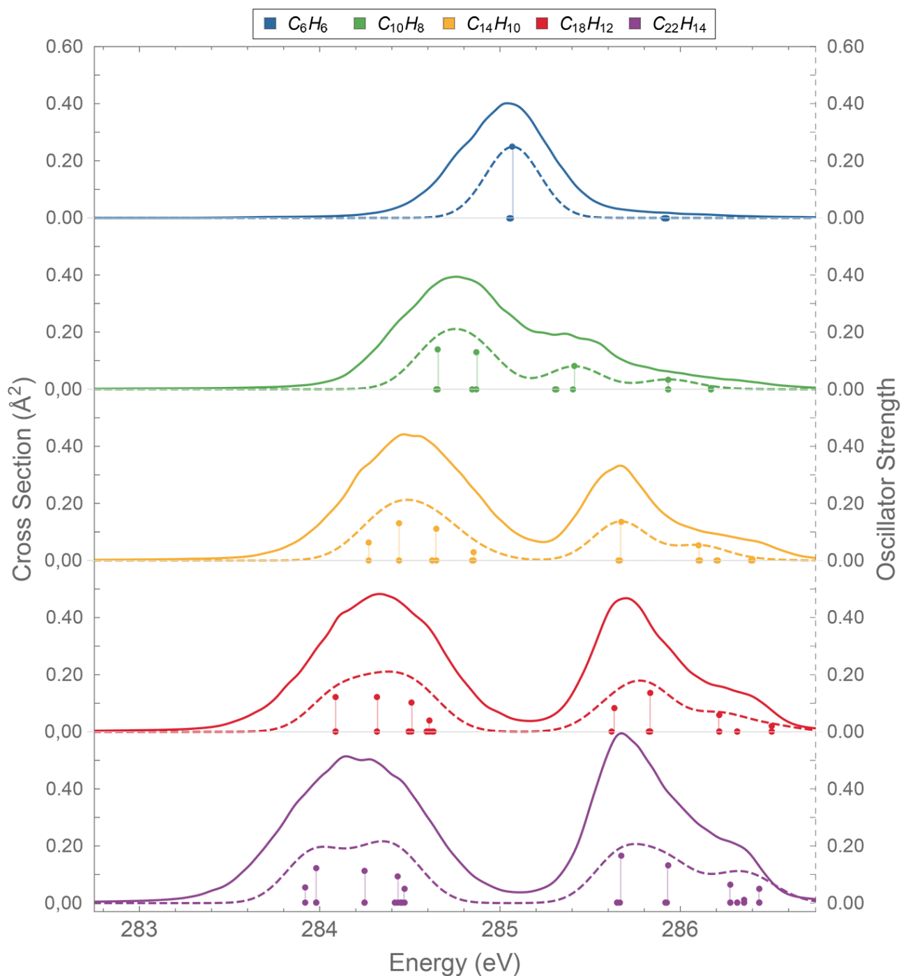
Figure 4. Calculated inner-shell spectra for carbon 1s at TD- \omega B97XD/ma-Def2-SVP level with Nuclear Ensemble method (full lines). Vertical lines show the transitions obtained at equilibrium geometry, with their spectra representation, using Gaussian functions with 0.30 eV width (dashed lines). All energy values are shifted by 9.3 eV.
