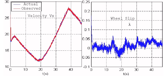
Fig. 9. Estimated velocity using the ABS sensors
