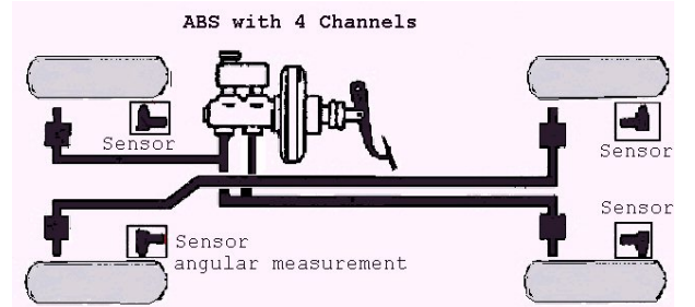
Fig. 4. 4 Sensors used by ABS 29dot/2 \pi
