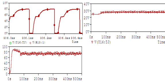
Figure 4.5: Effect of a deformation in PWM signal
