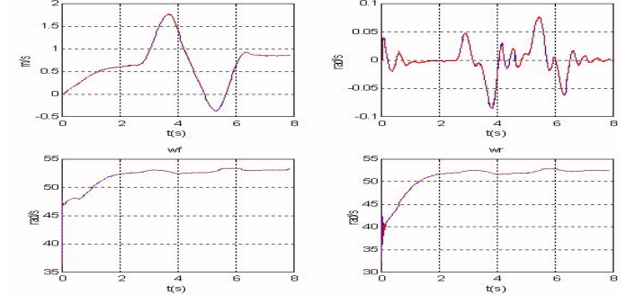
Fig. 5. Estimated and Measured States
