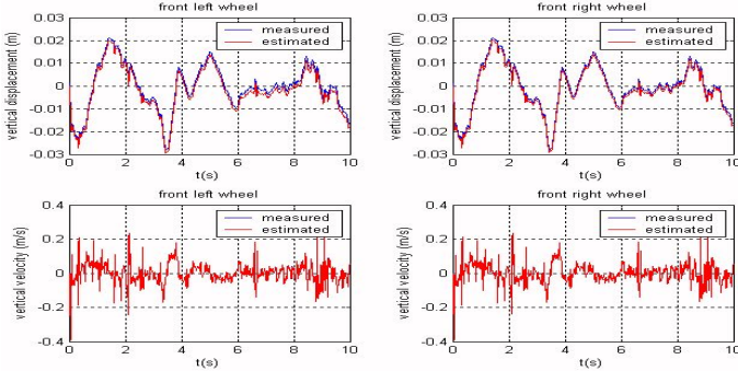
Fig. 8. Estimated and measured displacement of the wheels
