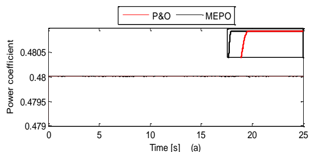
Fig.12. (a) C_p and (b) optimal and extracted power For [P&O MPPT, x=5 ]
