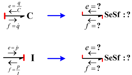
Figure 17. Substitution of storage ( I and C ) elements by bicausal double sources element.
