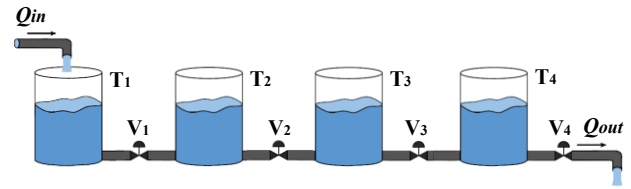
Figure 2. Four hydraulic tanks system.
