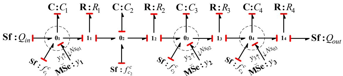
Figure 6. Diagnostic bond graph \tilde{\mathbf{B}} .
