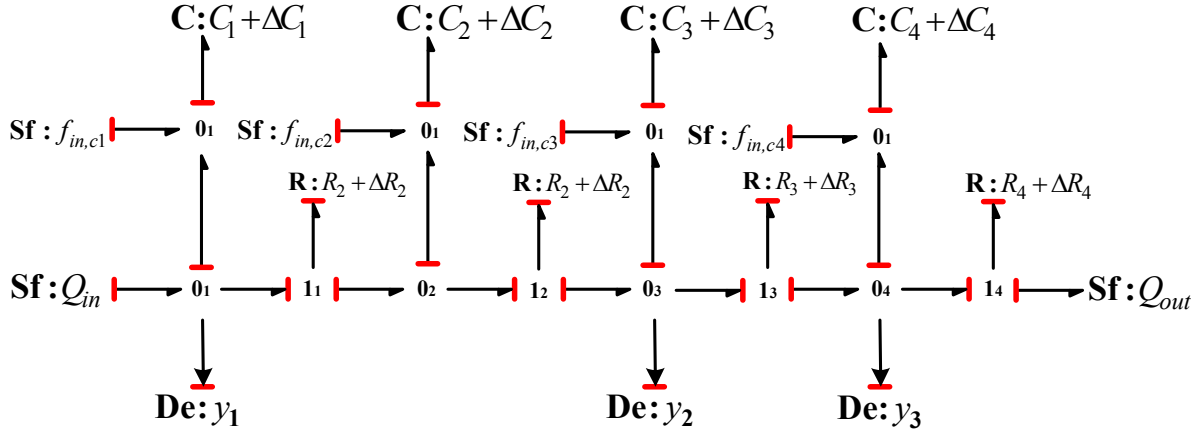
Figure 4. Faulty linearized bond graph \mathbf{B} in integral causality of the four hydraulic tanks system.
