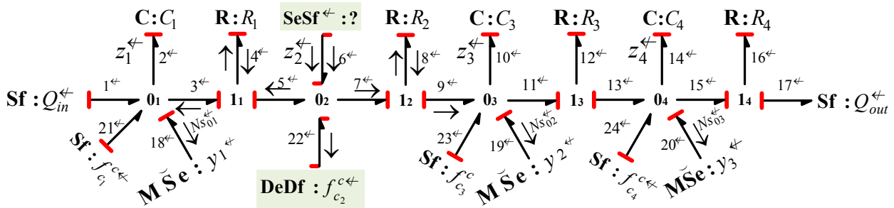
Figure 7. Decoupled bicausal DBG \tilde{\mathbf{B}}_{f_{c2}^c}^{c+} from the component fault f_{c2}^c .
