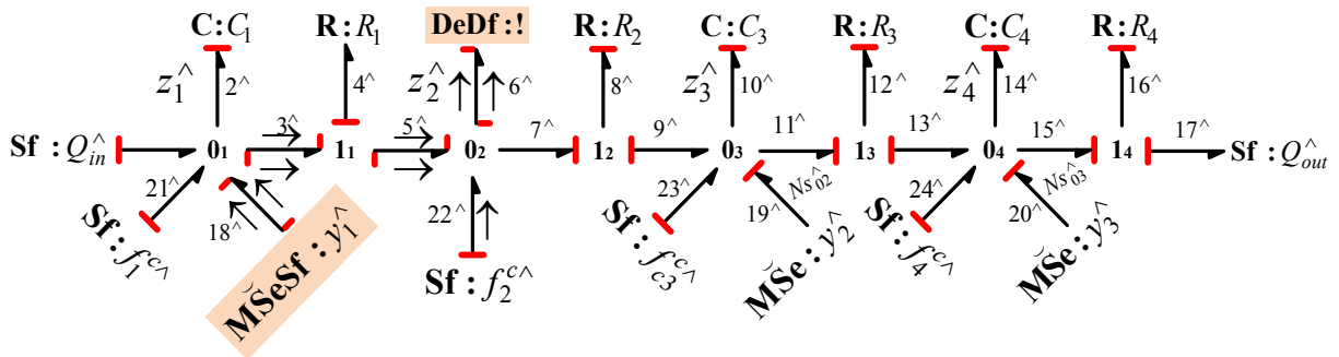
Figure 8. Estimator bicausal DBG \tilde{\mathbf{B}}_{f_{c_2}^c}^\wedge(z_2) for the structurally decoupled estimation
