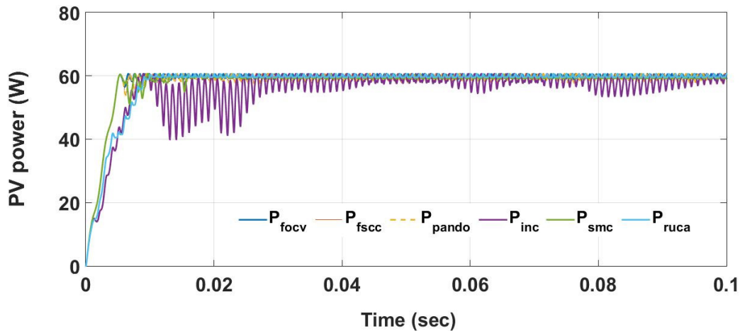
Figure 5. Simulation under standard condition: irradiation = 1000/\text{m}^2 and temperature = 25^\circ\text{C}
