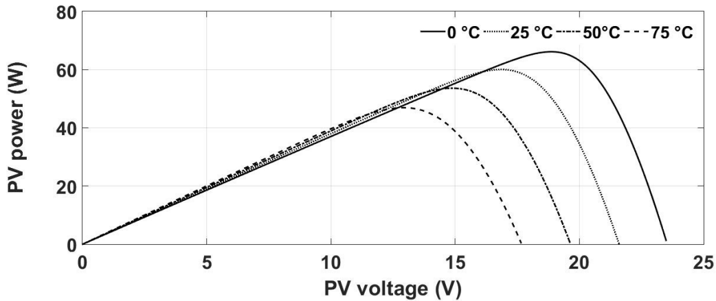
(a) Under different temperature values and fixed irradiation = 1000 \text{ W/m}^2
