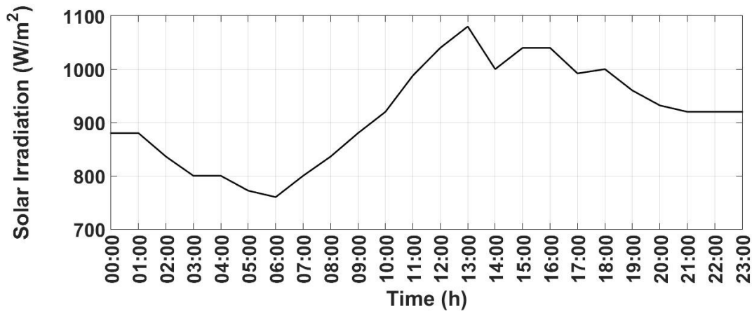
(a) Solar irradiance taken for a hot day
