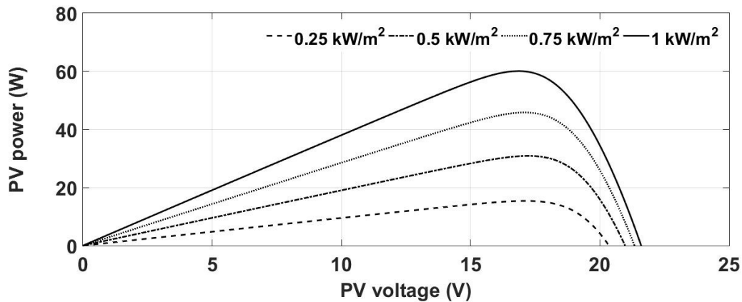
(b) Under different irradiation values and fixed temperature = 25^\circ\text{C}
