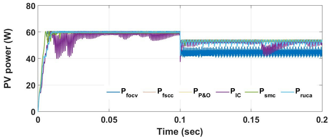
Figure 6. Simulation under step change of temperature: 25^{\circ}\text{C} \rightarrow 50^{\circ}\text{C} and fixed irradiation = 1000\text{W}/\text{m}^2
