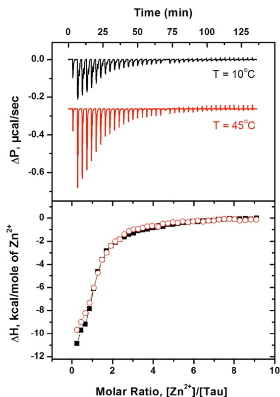
Fig. 2. Typical ITC titration curves (top panel) and binding isotherms (bottom panel) for zinc at 10^\circ\text{C} (black) and at 45^\circ\text{C} (red) interactions with 30\ \mu\text{M} of tau in 50\ \text{mM} Tris and 1\ \text{mM} TCEP at pH 7.5.
