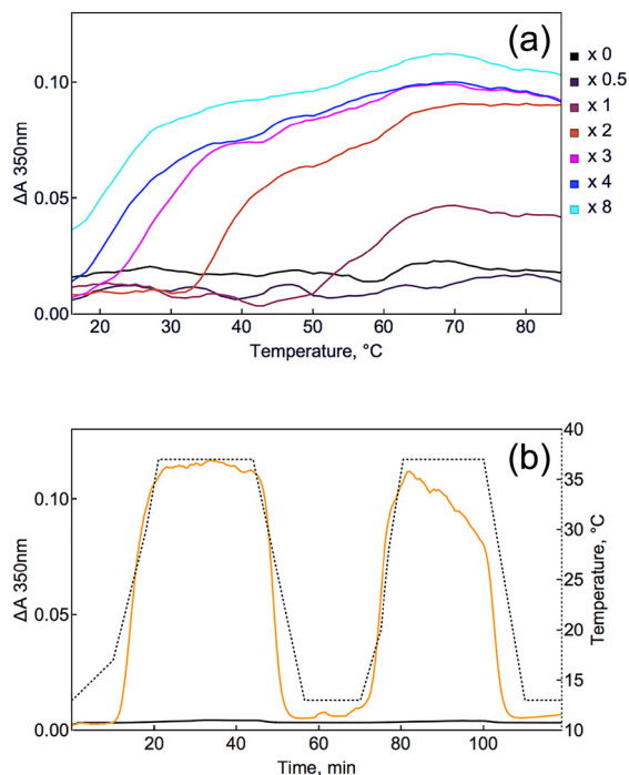
Fig. 1. (a) Temperature dependence of 30 \mu M tau samples turbidity in the absence of ZnCl_2 (black curve) and in the presence of 0.5-, 1-, 2-, 3-, 4- and 8-fold molar excess of ZnCl_2 (see color legend on the right) in 50 mM Tris buffer and 1 mM TCEP at pH 7.5 obtained using Prometheus NT.Plex instrument. (b) Reversible aggregation of tau (30 \mu M) followed by turbidimetry in the presence of 4-fold molar excess of ZnCl_2 (yellow curve); control tau sample in the absence of zinc (black curve); variation of temperature during experiment (black dotted line). Measurements were carried out using PerkinElmer spectrophotometer Lambda 800.
