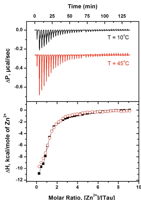
Fig. 2. Typical ITC titration curves (top panel) and binding isotherms (bottom panel) for zinc at 10 °C (black) and at 45 °C (red) interactions with 30 μM of tau in 50 mM Tris and 1 mM TCEP at pH 7.5.
