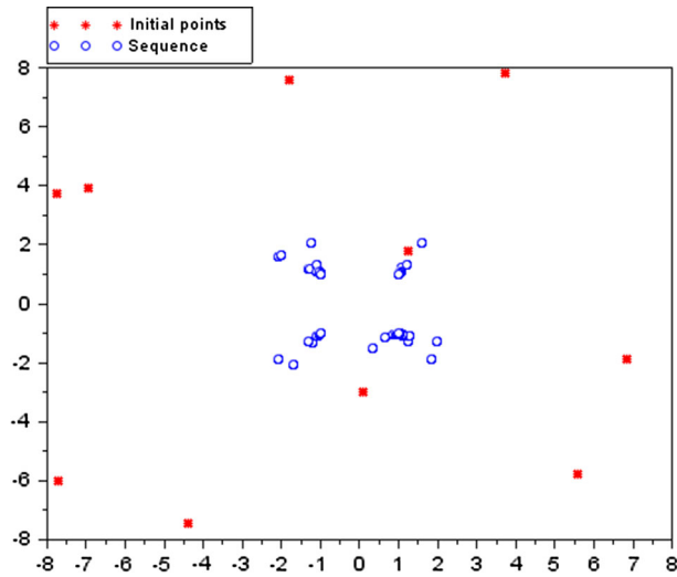
Fig.1 Algorithm running with 10 randomly starting points
