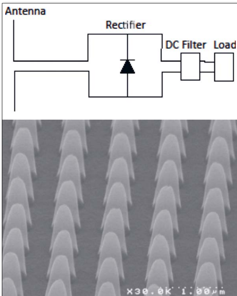
▼ FIG 3: (a) Schematic of a rectenna. (b) SEM image of nanopryramids obtained by nano-imprint lithography. [16]
