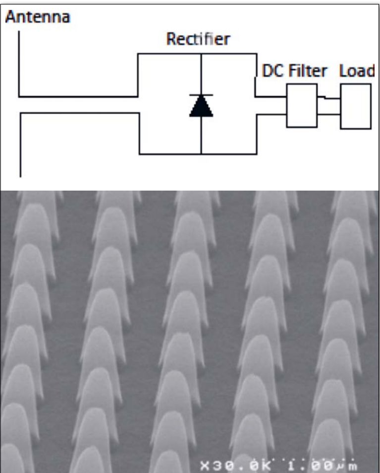
▼ FIG 3: (a) Schematic of a rectenna. (b) SEM image of nanopillar structures obtained by nano-imprint lithography. [16]
