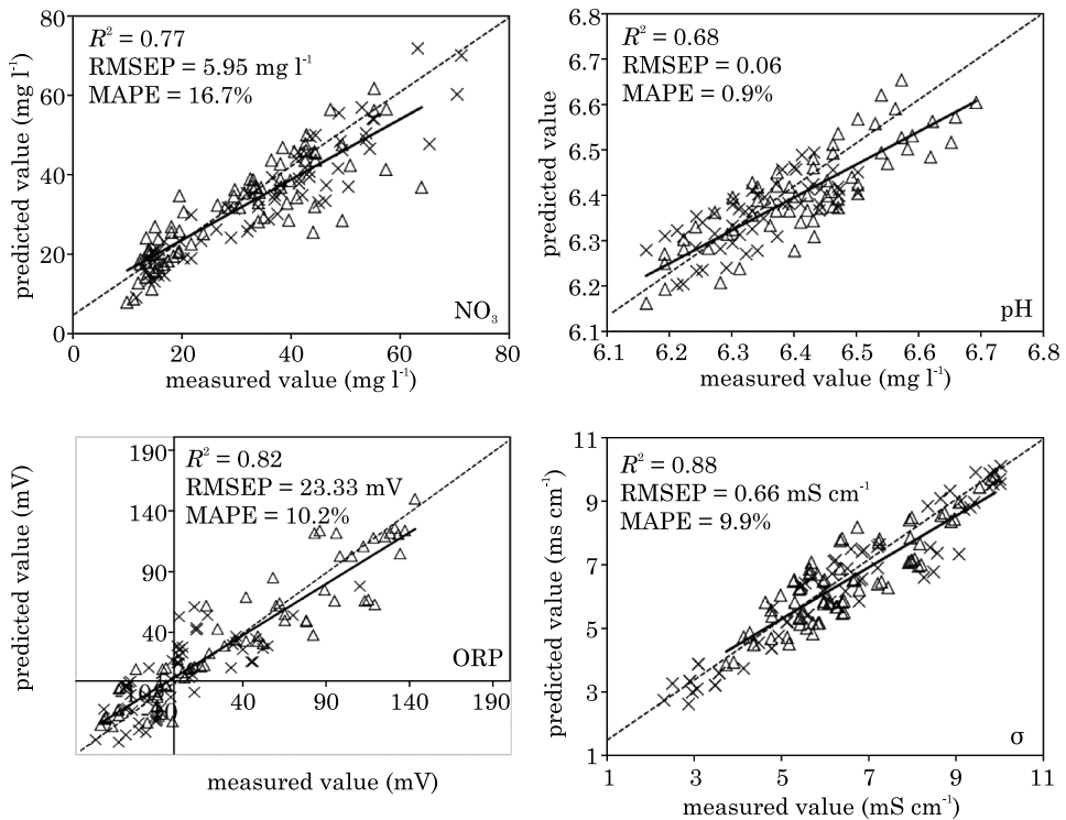
Fig. 1. Measured and predicted values of pH, ORP, \sigma and NO 3 , including the full spectral range of all investigated samples (residuals referring to conventionally grown samples are marked 'X', organically 'Δ')
